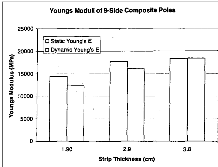
Figure 5. Comparisons between dynamic Young's moduli predicted by the free transverse vibration method and the static Young's moduli calculated from the measurement of strains in LCP members containing 9 trapezoid-shape strips.
