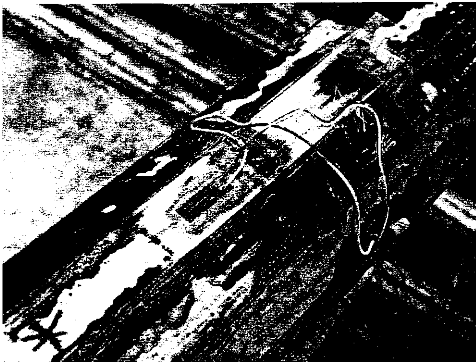
Figure 2. Strain gages were used to measure the strain and vibration frequencies of LCP.
