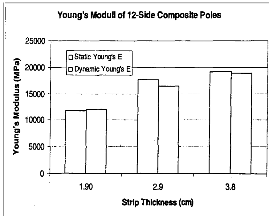
Figure 6. Comparisons between dynamic Young's moduli predicted by the free transverse vibration method and the static Young's moduli calculated from the measurement of strains of LCP members containing 12 trapizoid-shape strips.
