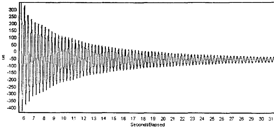
Figure 4. A typical vibration curve of a LCP tested under dynamic bending
