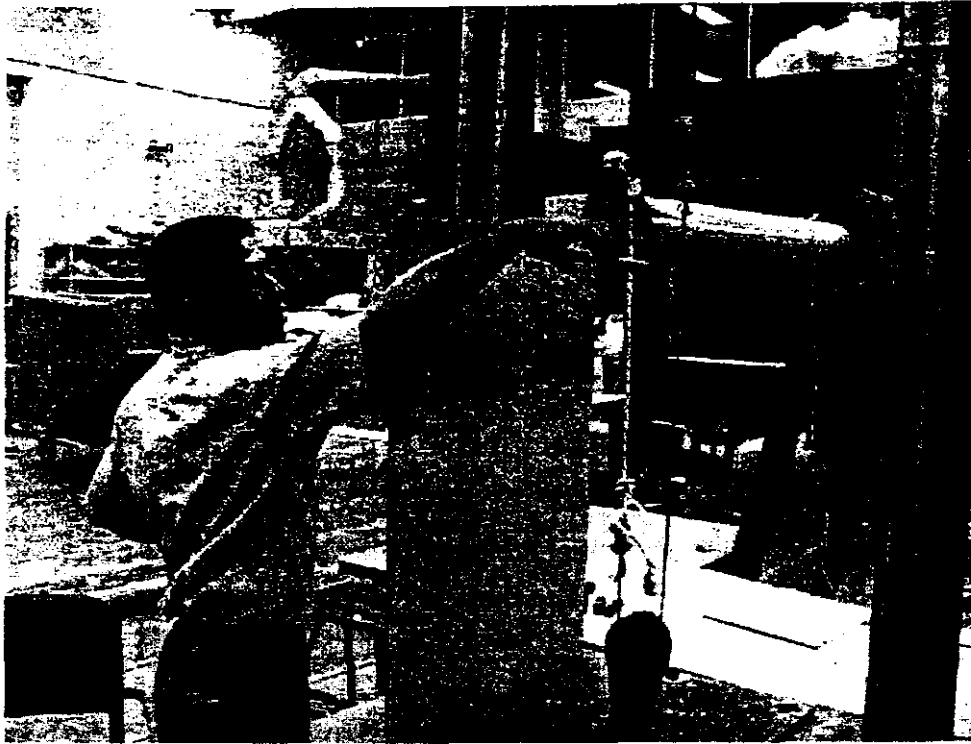
Figure 3. Rope cutting for generating a free vibration of LCP in a dynamic bending test.
