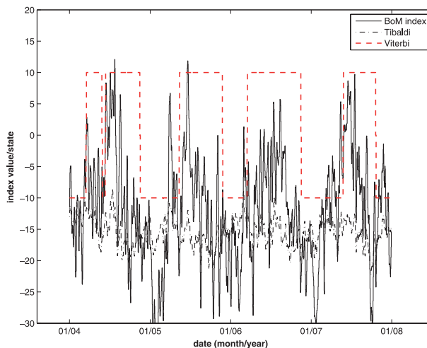
FIG. 17. As in Fig. 16, but with the Tibaldi index included and a nonzero smoothing (persistence parameter set to 100) set in the FEM-BV-VARX. This figure clearly displays the tendency of the AMIP simulation to lock into one state for long periods.
