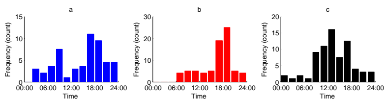
Fig. 3. Peak-time distributions for (a) Period 1 ( n = 37 ), (b) Period 2 ( n = 58 ) and (c) Period 3 ( n = 62 ), where n is number of constituent profiles. Where peaks straddled 2 time slots, each bi-hourly bin was assigned a value of 0.5.
