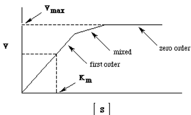
Fig. 8. A Michaelis-Menten plot.
