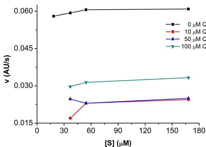
Fig. 13. Lipoxygenase inhibition by quercetin at different concentrations (10 \mu\text{M} , 50 \mu\text{M} and 100 \mu\text{M} ). Protocol 1 (Fig. 10) was followed for measurements as indicated in the legend of Fig. 11.
