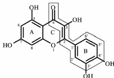
Fig. 7. Chemical structure of quercetin. Frame highlights the cinnamoyl part of the molecule (Zsila et al., 2003).
