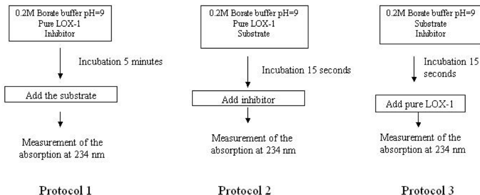
Fig. 10. Schematic representation of experimental protocols (1,2,3).
