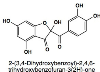
Fig. 5. Product of oxidative degradation of quercetin by soybean LOX-1 as proposed by Ha et al. (2010).
