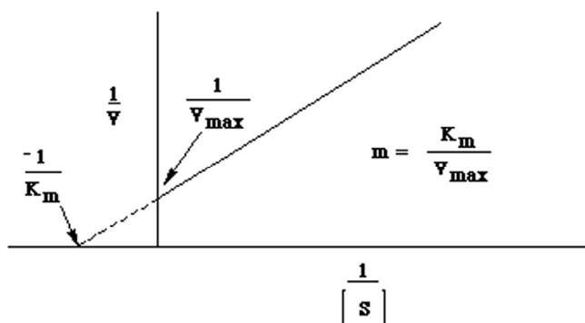
Fig. 9. A typical Lineweaver-Burk plot.
