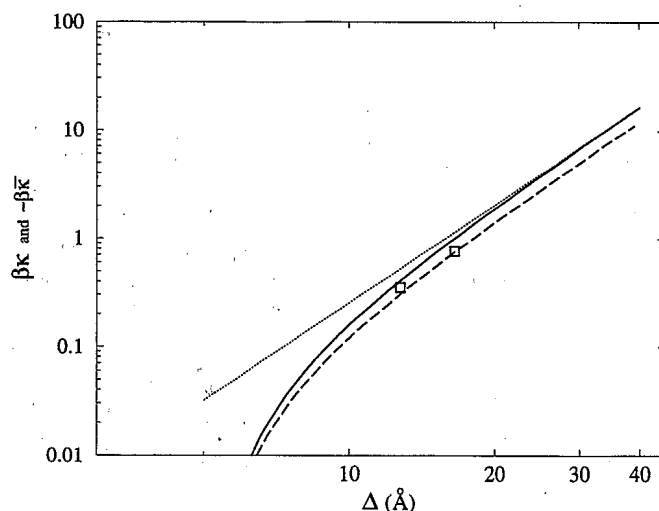
FIG. 2. The bending rigidity \kappa (solid line) and minus the saddle splay modulus -\bar{\kappa} (dashed line) of saturated monolayers as a function of surfactant chain length \Delta at \beta J=0.2 and a=2 \text{ \AA} . The thin dotted line has the slope 3 which represents the asymptotic scaling \kappa \sim \Delta^3 . The two rectangles represent the data points of bending rigidity from Ref. [16].
