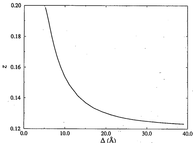
FIG. 1. The minimum of fugacity necessary to saturate the interface z_s as a function of chain length \Delta at \beta J=0.2 and a=2 \text{ \AA} .
