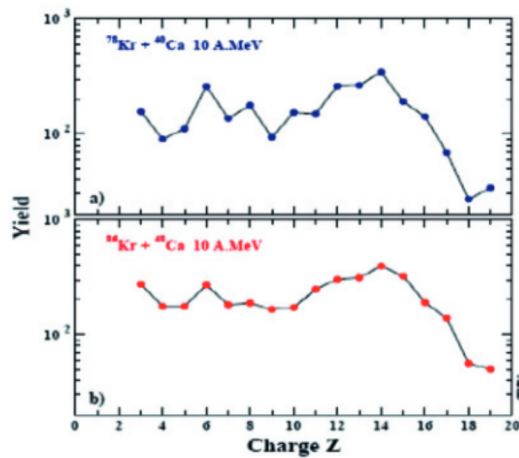
Figure 3: Charge yield of IMF for the n-poor system and the n-rich one, \theta = 10^\circ - 13^\circ .
