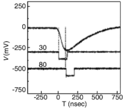
Figure 1: Signal rise-time as deduced by time difference between CFD's output at 30% and 80% of original signal.
