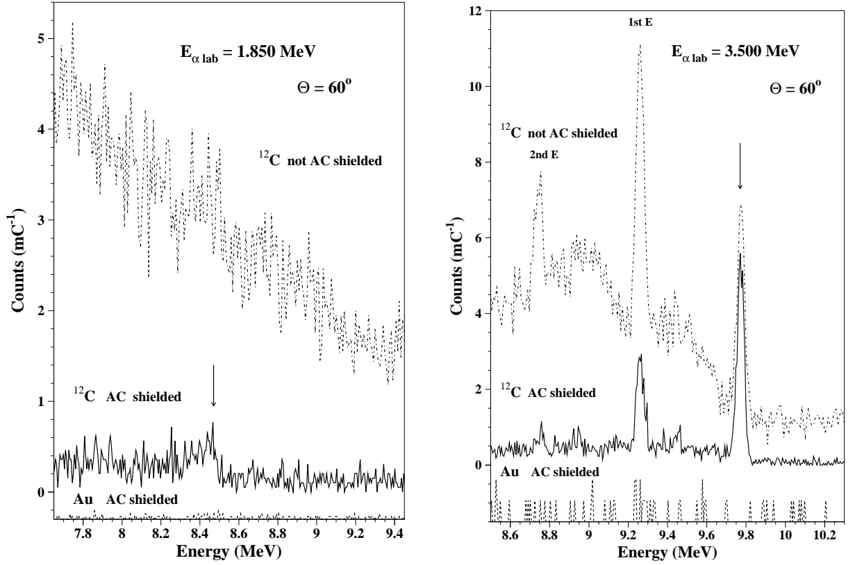
FIG. 4: \gamma -ray spectra of the ^{12}\text{C}(\alpha, \gamma)^{16}\text{O} reaction registered at 60^\circ for E_{\alpha, \text{lab}} = 1.850 \text{ MeV} , the lowest energy in this experiment, and E_{\alpha, \text{lab}} = 3.500 \text{ MeV} . The spectra at the top of the graphs were taken without Compton suppression, i.e. no active shielding. The spectra in the middle correspond to those with active shielding, and the spectra at the bottom represent the background measured with the beam on the bare gold backing. AC means Compton suppression. For better clarity, the two lower spectra are shifted by -0.3 and -1.5 on the y-axis. Peaks of interest are indicated by arrows. The symbol 1st E (2nd E) indicates the first (second) escape peak. All spectra are normalized to the accumulated charge (counts per milli Coulomb of \alpha -particle beam).
