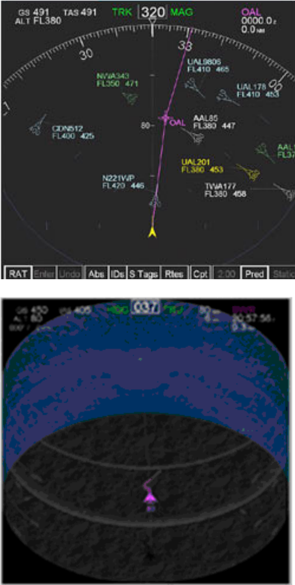
Figure 2.21. Potential Cockpit Display of Traffic Information (CDTI) may be implemented as 2-D (top), or 3-D (bottom) (source: http://humansystems.arc.nasa.gov/ihh/cdti/cdti.html )
