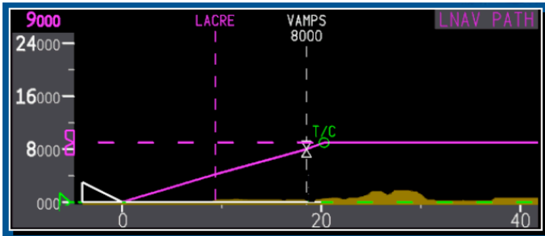
Figure 2.19. A Potential Vertical Situation Display. Source: Carriker, 2006.
