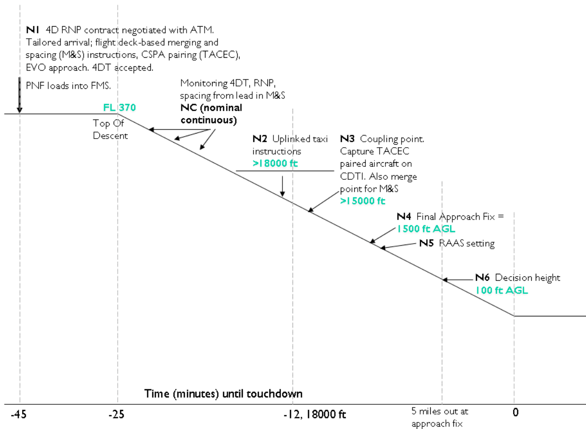
Figure 2.22. Nominal Event NextGen Approach/Arrival Scenario
