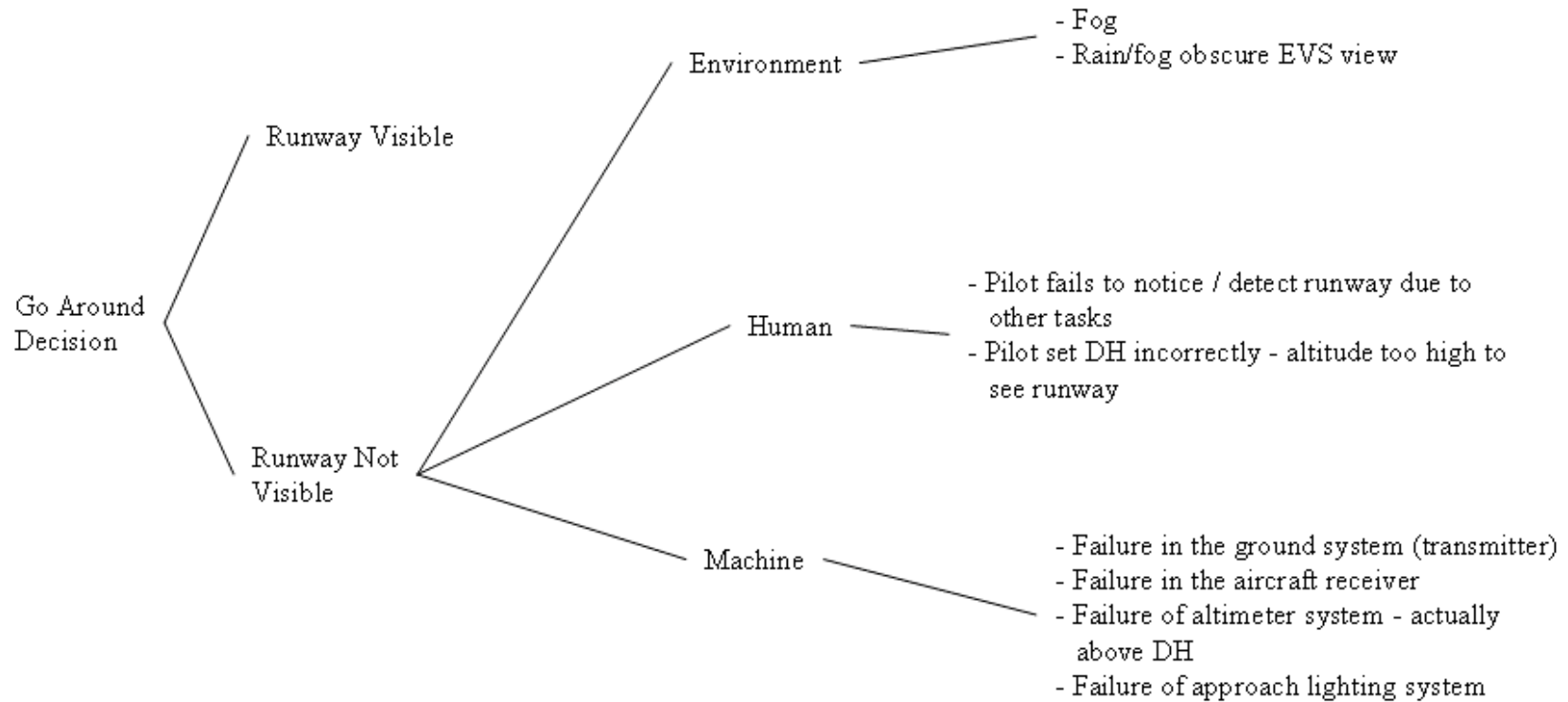
Figure 2.32. Murphy Diagram of NextGen Arrival / Approach Off-Nominal 9
