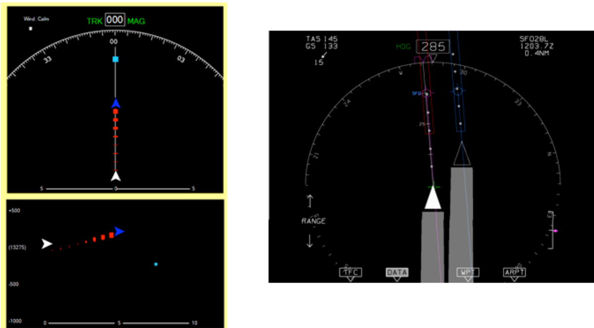
Figure 2.20. Potential Wake Vortex Displays (from Sebok et al., 2006, left, and Hardy & Lewis, 2004, right)
