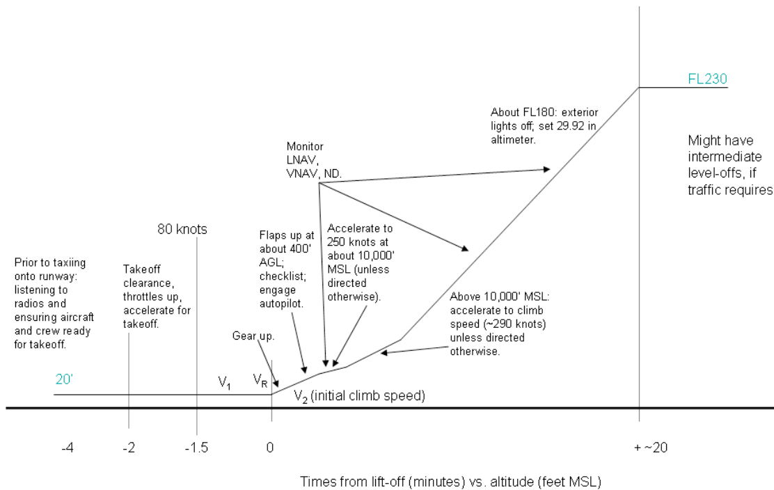
Figure 2.11. Current-day Departure Scenario
