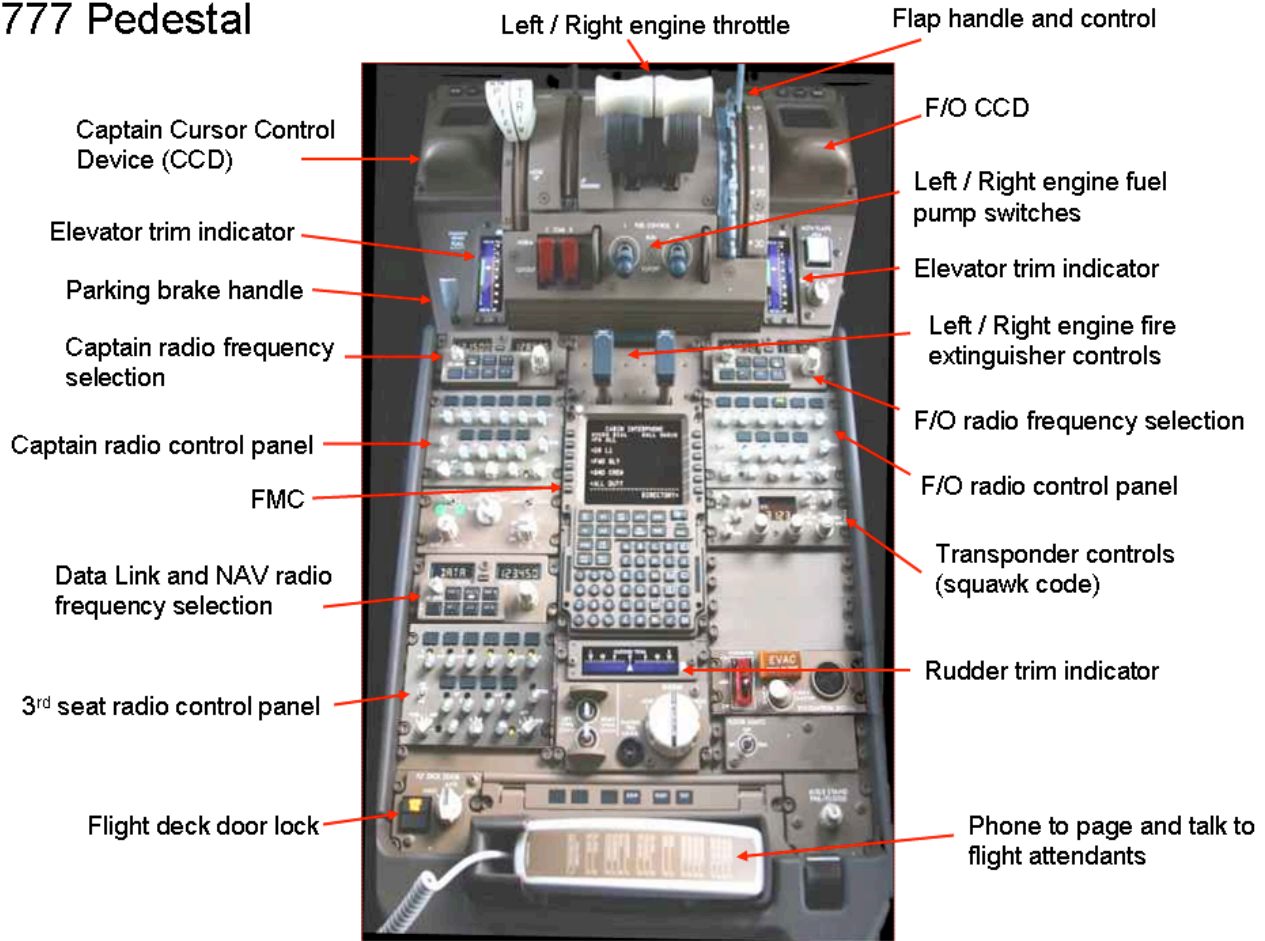
Figure 2.9. A B-777 Pedestal
