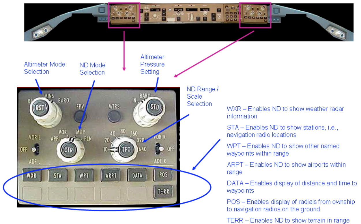
Figure 2.7. The Electronic Flight Instrument System
