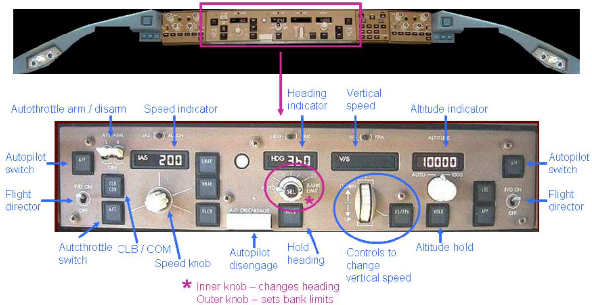
Figure 2.4. A B-777 Mode Control Panel
