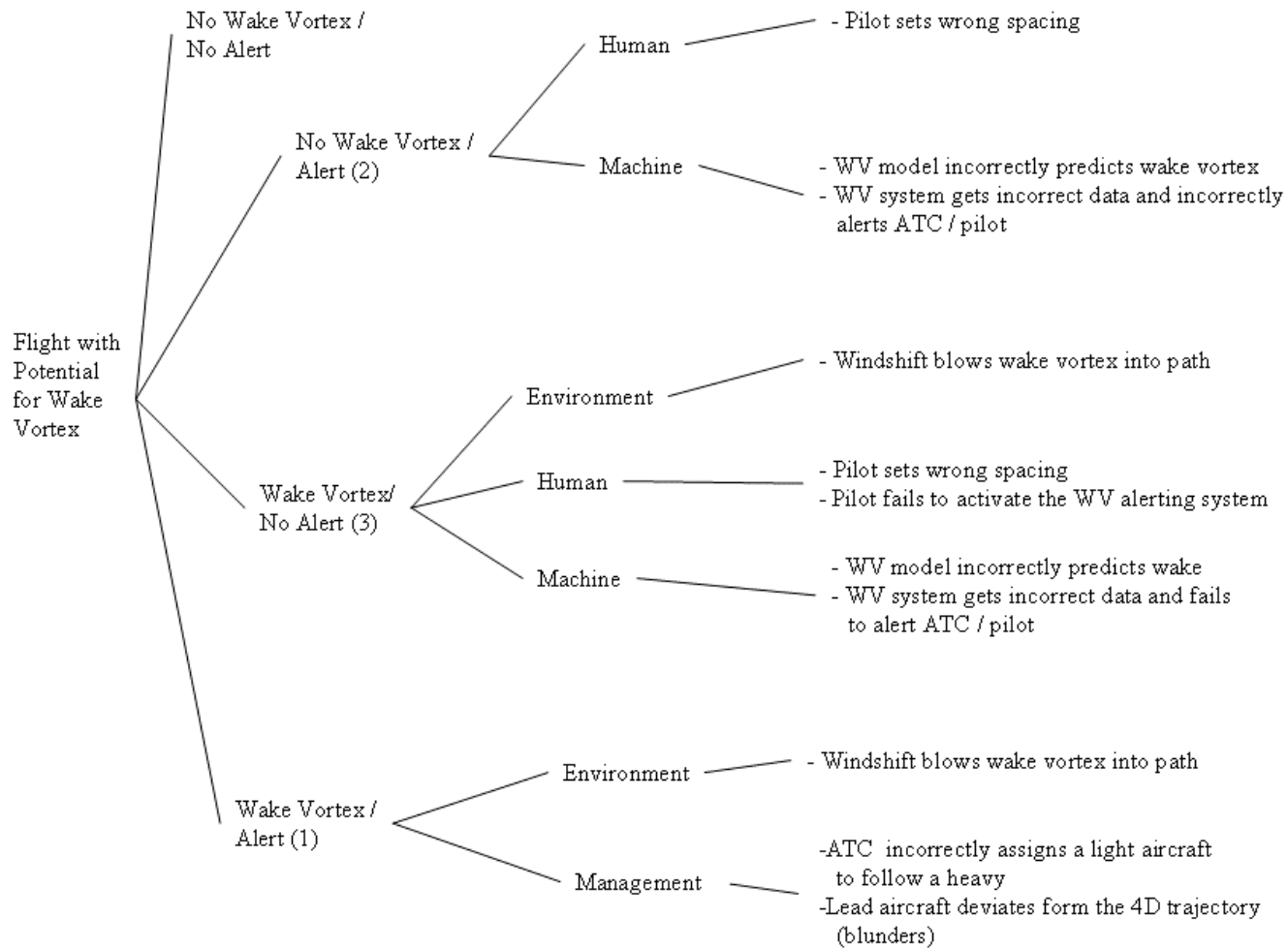
Figure 2.29. Murphy Diagram of NextGen Arrival / Approach Off-Nominal 6
