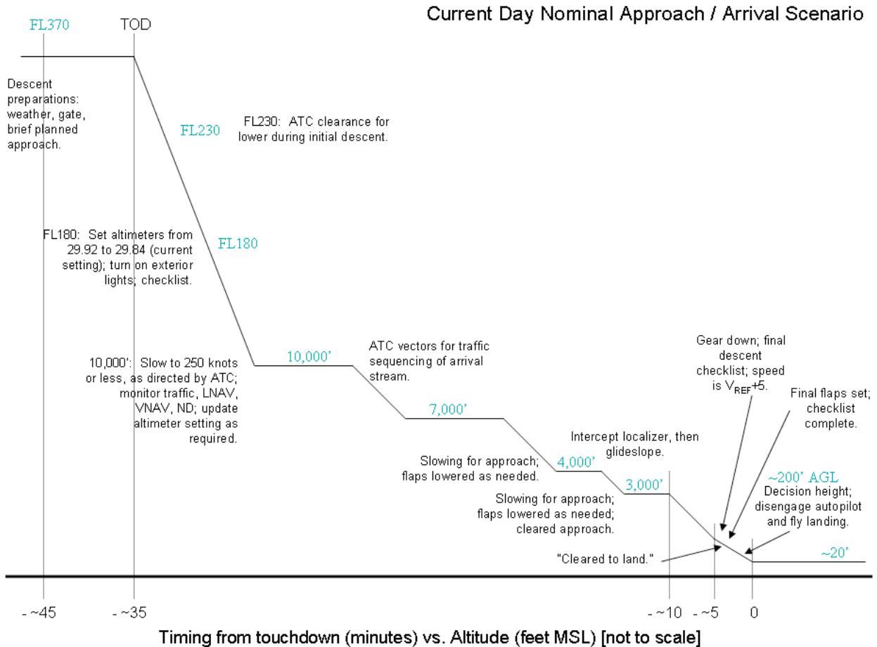
Figure 2.10. Current-day Nominal Arrival Scenario
