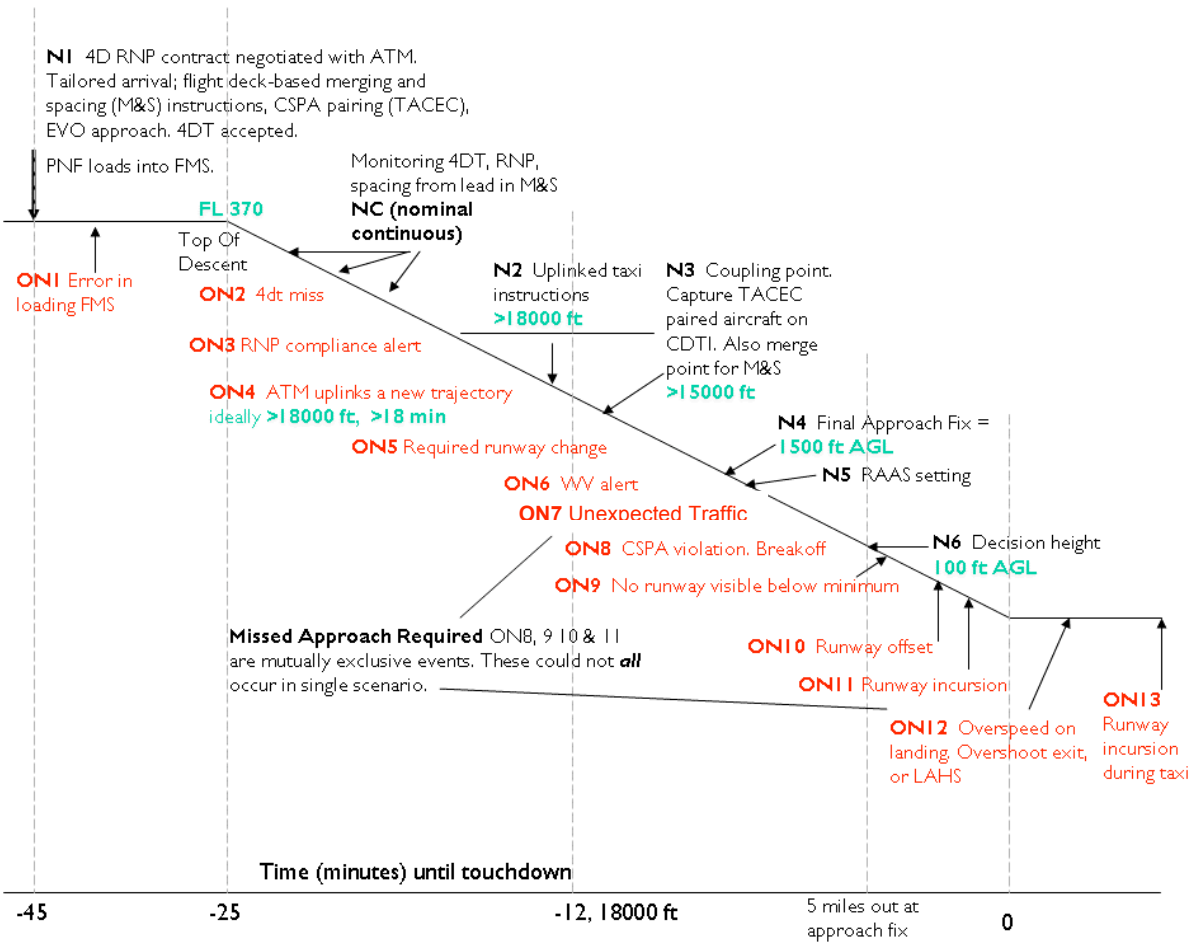
Figure 2.23. A NextGen Arrival Scenario with Nominal and Off-Nominal (ON) Events
