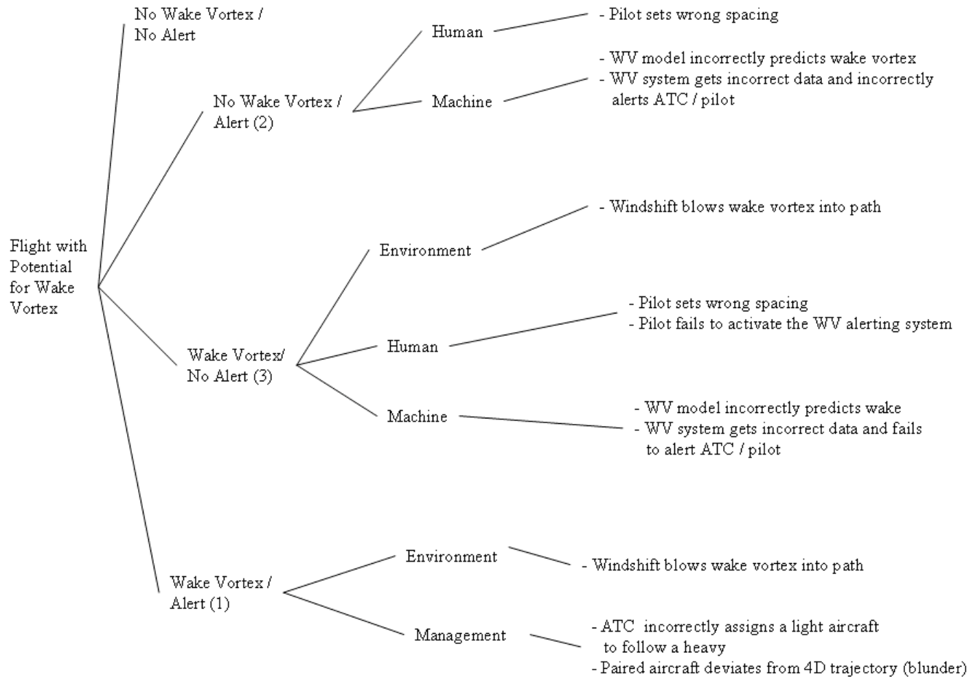
Figure 2.45. Murphy Diagram of NextGen Departure Off-Nominal 7
