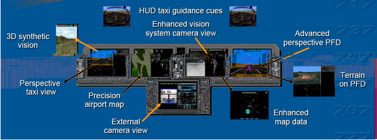
Figure 2.15. A Boeing 787 Flight Deck Layout, Including a Synthetic Vision System, an Enhanced Vision System (Camera Views), Taxi Guidance, and Terrain Data on the PFD. Source: Carriker, 2006.
