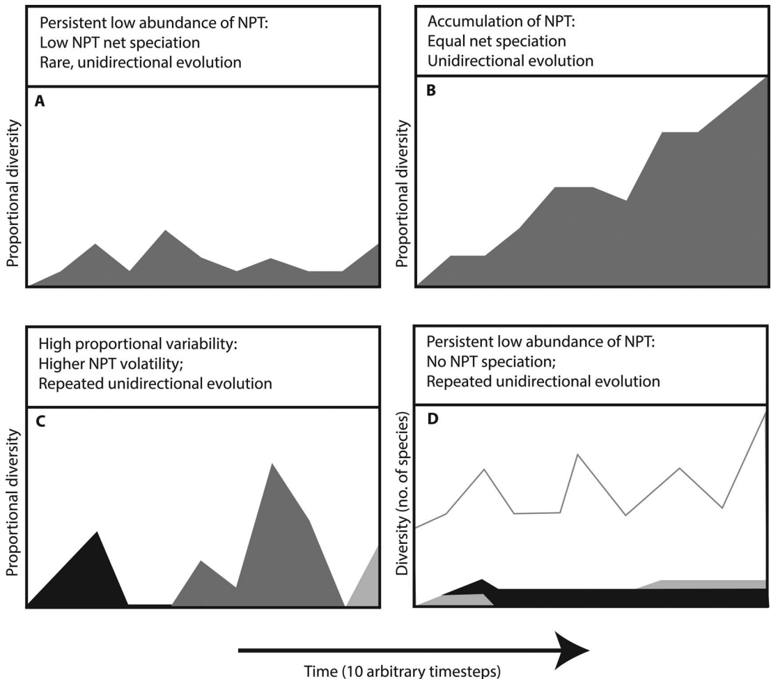
FIGURE 1. Proposed effects of non-planktotrophy on the proportion of planktotrophic (PT) taxa (white) to non-planktotrophic (NPT) taxa (filled) based on speciation and extinction rates in four theoretical models of macroevolution. A, Rare origins of new non-planktotrophic lineages from planktotrophic taxa coupled with low speciation rates lead to persistence at low relative diversity. B, Non-planktotrophic lineages of equal or higher net speciation than planktotrophic lineages accumulate passively due to the one-way nature of the transitions. C, Non-planktotrophic lineages with higher rates of both speciation and extinction due to their low population sizes and low connectivity would result in strong fluctuations of relative diversity, with frequent extinction of non-planktotrophic lineages. D, For non-planktotrophic lineages with extremely low speciation rates, the total diversity is dictated by the frequency of new non-planktotrophic lineages from planktotrophic taxa relative to extinction rate.
