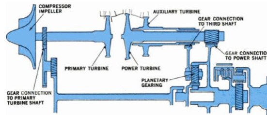
Figure 6: Layout of turbine M-M shafts and planetary M-M gears for the KTT three-stage AGT [1].
