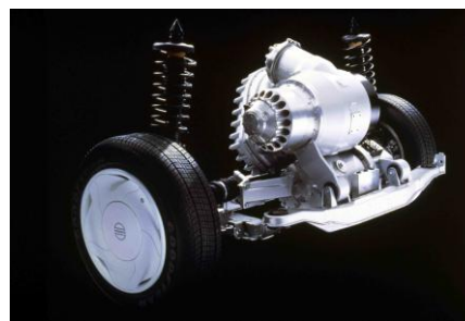
Fig. 4: Volvo ECC's AGT/M-E generator to power the serial HEV's E-M motor [5]
