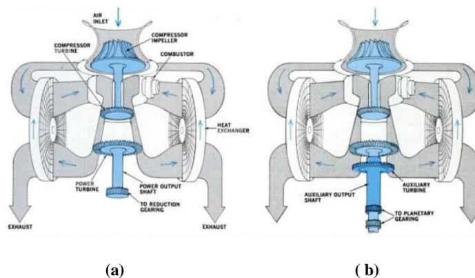
Figure 5: Conventional two-stage AGT (a) and KTT three-stage AGT (b). [1].
