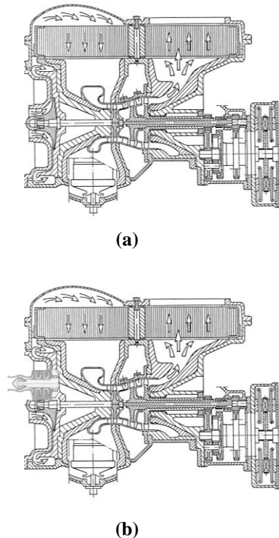
Figure 8: Layouts of turbine M-M shafts and planetary M-M gears for the VZE three-stage AGT that is based on the FTB system with the M-P compressor (a) or M-F pump (b) [4].
