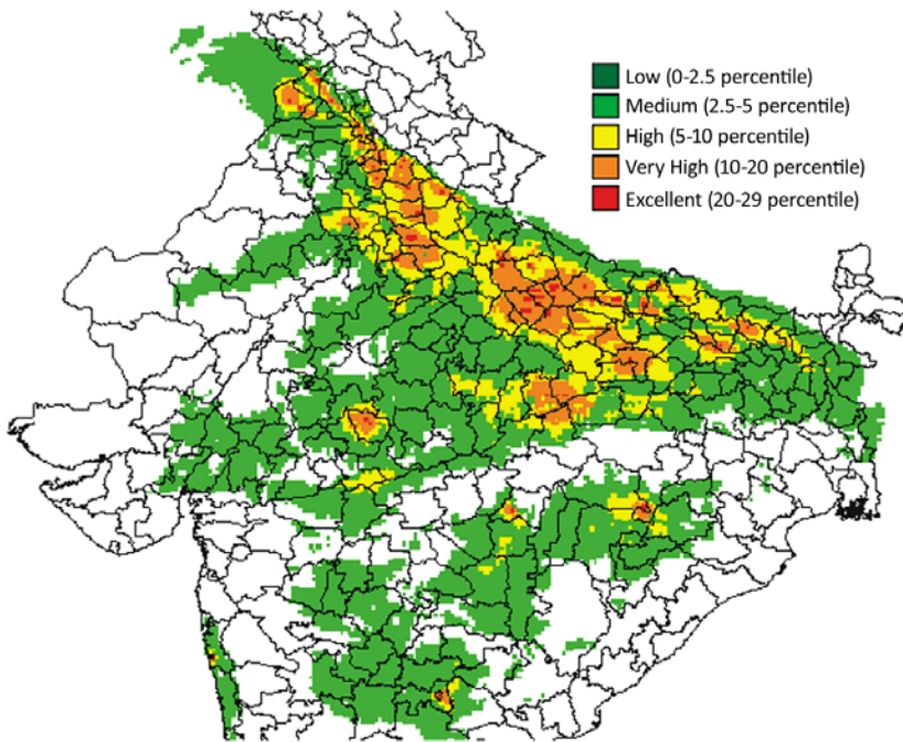
Figure 1. Climate suitability map for Dussaheri mango.
