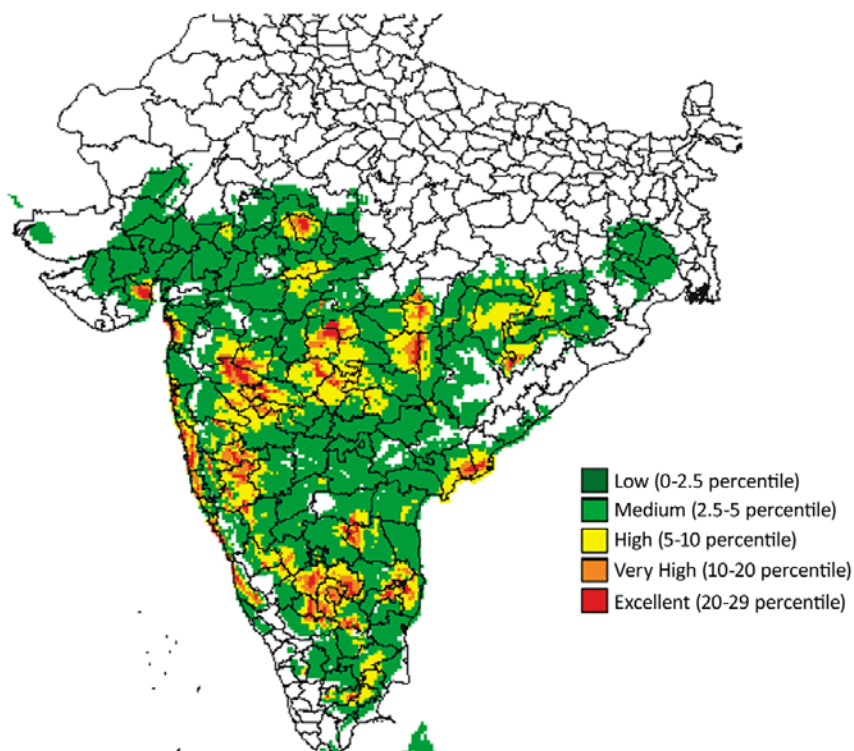
Figure 2. Climate suitability map for Alphonso mango.
