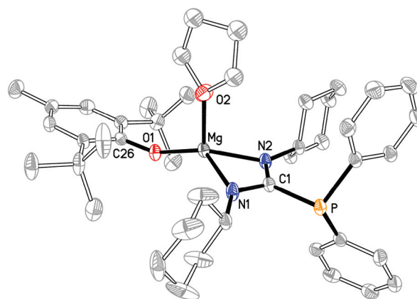
Fig. 6 Thermal ellipsoid plot (30% probability) of Mg(Ph 2 PC(NCy) 2 )-(OAr')(THF) 12 (hydrogen atoms omitted).
