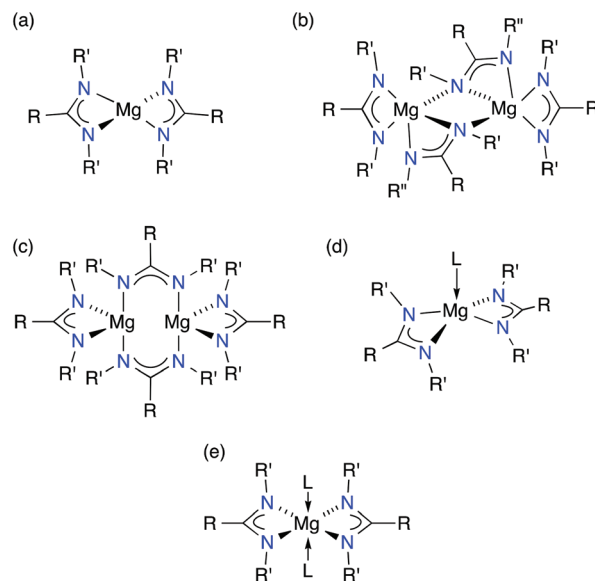
Fig. 8 Different structural types reported for \text{Mg}(\text{N}\langle\text{N}\rangle)_2(\text{L})_n .
