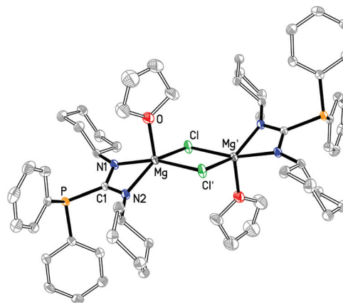
Fig. 4 Thermal ellipsoid plot (30% probability) of [Mg(Ph 2 PC(NCy) 2 )Cl](THF) 2 ( 6 ) 2 (hydrogen atoms omitted).
