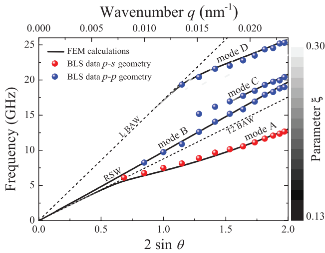
FIG. 3. Dispersion relation of SAWs propagating in [110] direction of a 1D surface phononic crystal. BLS experimental data (full circles) compared with FEM calculations (lines). Dashed lines show corresponding dispersion relations of longitudinal (L BAW), slower transverse (T2 BAW) bulk waves and Rayleigh surface wave (RSW) typical for Si.
