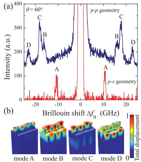
FIG. 2. (a) BLS spectra of a 1D surface phononic crystal for p - p and p - s geometry. (b) Corresponding FEM 3D deformation fields obtained for SAWs propagating in the [110] direction (parallel to the stripes) at q = 0.020456 nm -1 .
