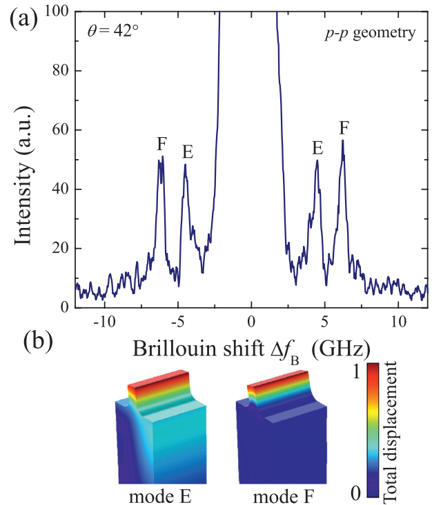
FIG. 4. (a) BLS spectra of a 1D surface phononic crystal for p - p geometry. (b) Corresponding FEM 3D deformation fields obtained for SAWs propagating in the [1\bar{1}0] direction (normal to the stripes) at q = 0.014542 \text{ nm}^{-1} .
