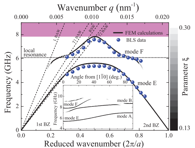
FIG. 5. Dispersion relation of SAWs propagating [1\bar{1}0] direction of a 1D surface phononic crystal. BLS experimental data (full circles) compared with FEM calculations (lines). Dotted lines show the corresponding dispersion relations of longitudinal (L BAW), transverse (T1 BAW and T2 BAW) bulk waves, and Rayleigh (RSW) surface waves typical for Si. The inset presents the calculated angular dispersion of SAWs at q = 0.0105 \text{ nm}^{-1} .
