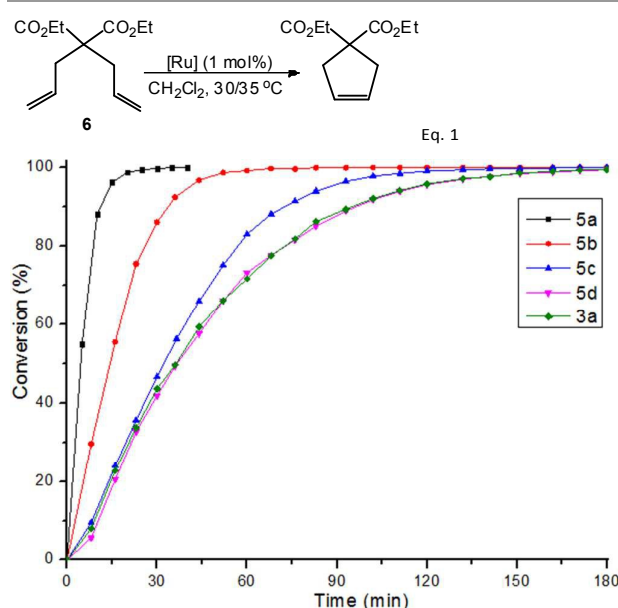
Fig. 4 The RCM of substrate 6 using 1 mol% of the complexes at 35 °C in CH 2 Cl 2 (1 M). The lines are intended as visual aid.
