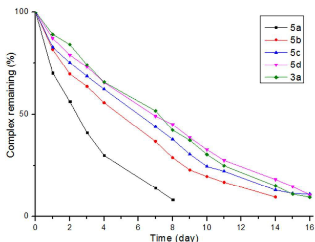
Fig. 3 Degradation of complexes 3a and 5a-d in a CDCl 3 solution at 20 °C in air measured by 1 H-NMR employing bis(3,5-dimethoxyphenyl)methane as an internal standard. The lines are intended as visual aid.
