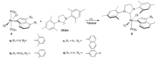
Scheme 1 Synthesis of complexes 5a-d from complexes 4a-d .
