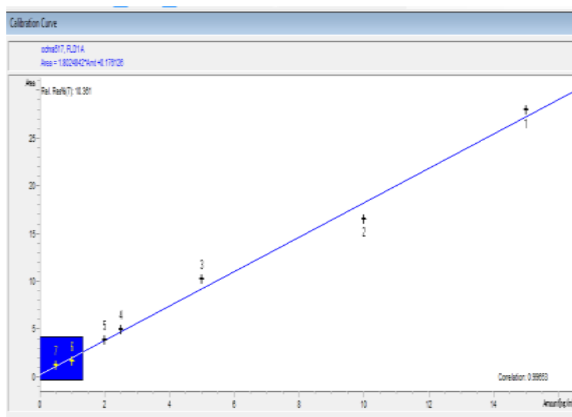
Figure 1: Calibration curve of standard solutions of OTA with concentrations of 0.5, 1, 2, 2.5, 5, 10 and 15 ppb by high-performance liquid chromatography analysis
