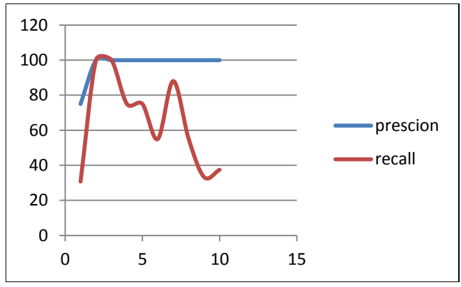
Figure 14. the relation between the Precision and the Recall
