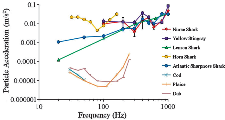
Fig. 1 Particle motion audiogram describing hearing thresholds of elasmobranch and teleost fishes. Modified from Casper and Mann (2009) and Fay (1988)
