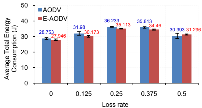
Fig. 6 Average total energy consumption vs. loss rate
