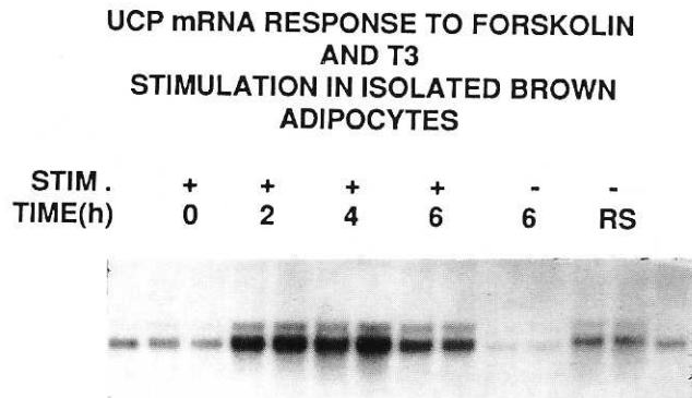
FIG. 1. Stimulation of UCP mRNA levels by forskolin and T 3 in dispersed brown adipocytes obtained from euthyroid rats. Northern blot of brown adipocyte RNA probed with 32 P-labeled UCP cDNA. Cells were obtained from euthyroid rats, as described in Materials and Methods , and incubated for the indicated times with 1 \mu M forskolin and 50 ng T 3 /ml. Cells from triplicate incubations (total, \sim 9 \times 10^6 ) were pooled and subjected to the RNA extraction procedure described in Materials and Methods . Each lane was loaded with 2 \mu g total RNA. The extreme left and right lanes were loaded with 2 \mu g total BAT RNA from euthyroid rats exposed to cold overnight. RS, Recovery standard; each of these lanes were also loaded with 2 \mu g RNA from an identical number of cells that were directly lysed in guanidinium thiocyanate without being submitted to any of the manipulations of the cells undergoing the incubation. Densitometric data are given in Results .
