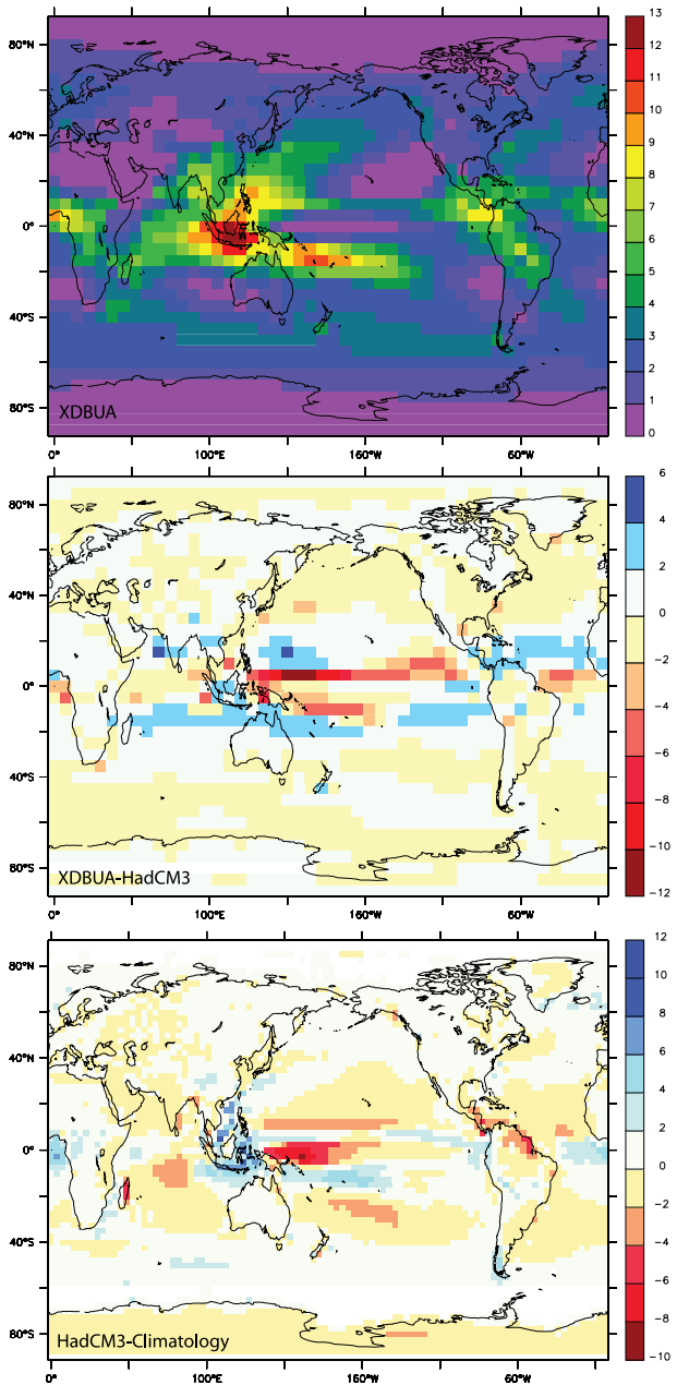
Fig. 7. Annual average precipitation (mm/day). Top: XDBUA; middle: XDBUA-HadCM3; bottom: HadCM3-CMAP (Xie and Arkin, 1997).
