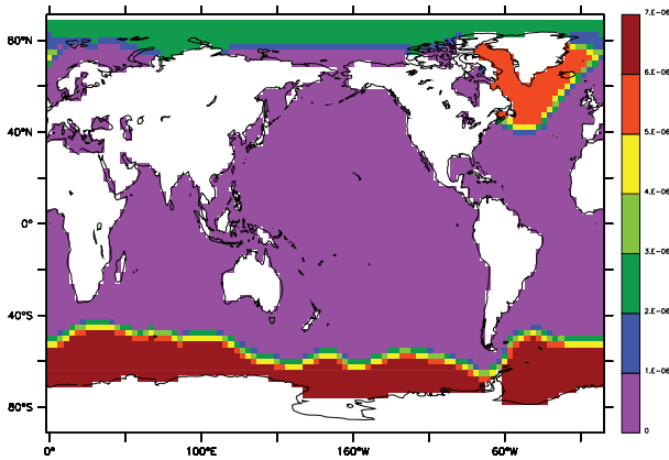
Fig. 2. Water flux ( \text{kg/m}^2/\text{s} ) applied to the ocean as a simple iceberg calving parameterisation to balance the build up of snow on ice sheets.
