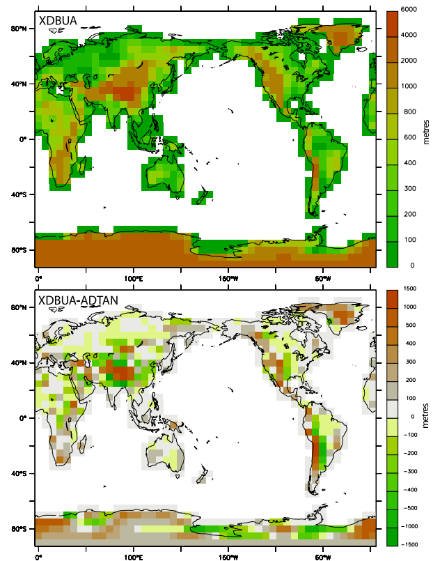
Fig. 1. Land orography used in XDBUA. Above: height above sea-level (metres) for all land points, including coastally tiled gridboxes that are considered partially ocean by the atmosphere model; below: difference (metres) from the orography used in ADTAN.
