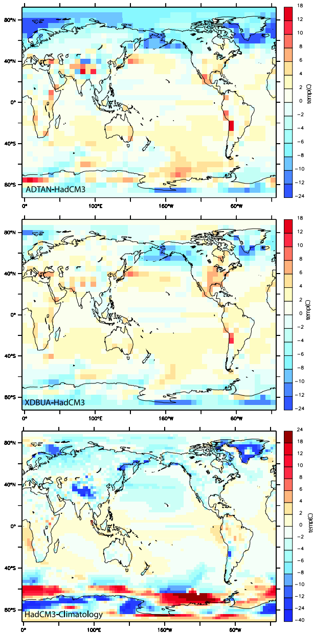
Fig. 6. Annual average surface temperature differences ( ^{\circ}\text{C} ). Top: ADTAN-HadCM3; middle: XDBUA-HadCM3; bottom; HadCM3-Legates and Willmott (1990).
