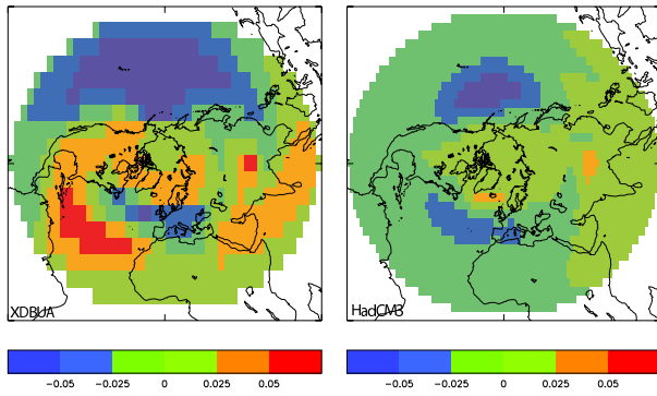
Fig. 9. The leading EOF of annual mean sea level pressure in (left) XDBUA and (right) HadCM3. They explain 21% and 25% respectively of the total variability in each model.
