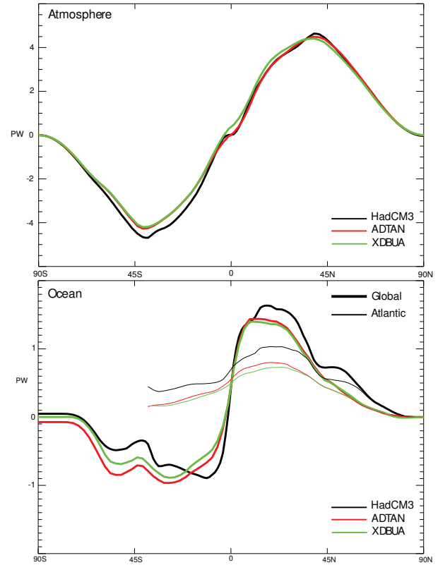
Fig. 11. Above: Atmospheric energy transport (PW). Black: HadCM3; Red: ADTAN; green: XDBUA. Below: Ocean heat transports (PW). thin line: Atlantic; thick line: Global. Colours as above.
