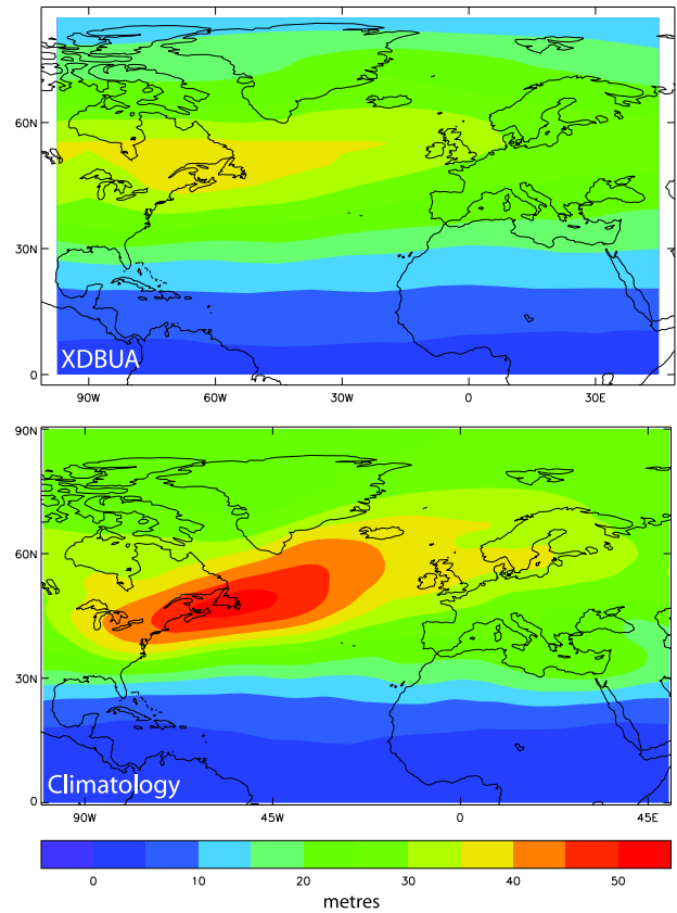
Fig. 8. 500 mbar geopotential height anomalies, 2–6 day bandpass filtered (metres). Top: XDBUA; bottom: ERA-40 (Uppala et al., 2005).
