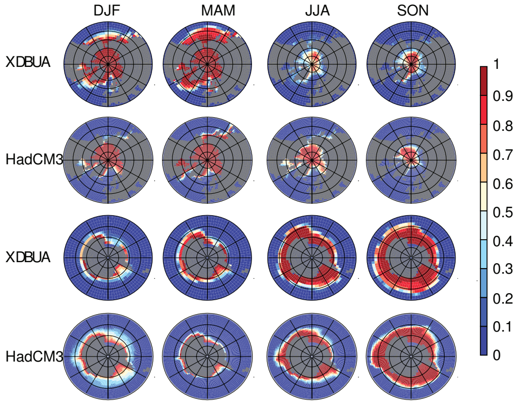
Fig. 4. Seasonal average ice gridbox fractions, XDBUA and HadCM3. Top two rows Northern hemisphere; bottom two rows Southern Hemisphere.
