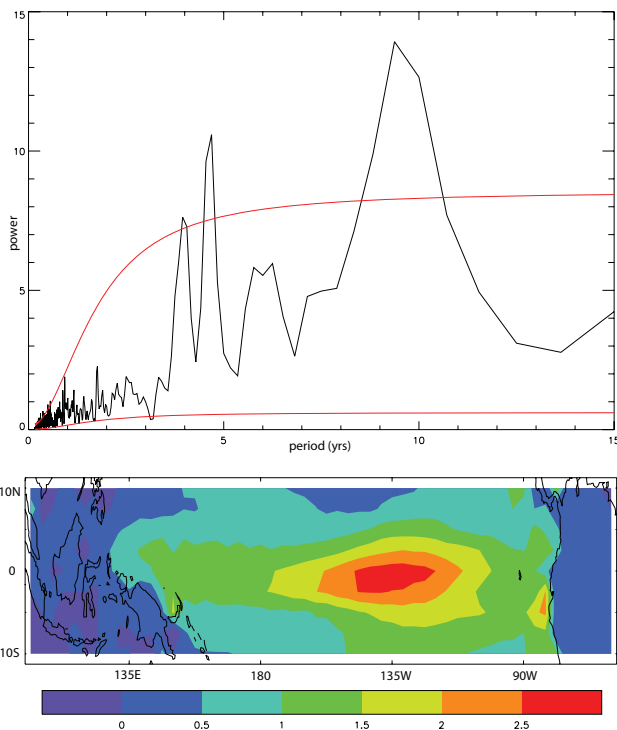
Fig. 10. Above: Power spectrum of 150 years of a Nino3 index from XDBUA (black). Red lines show 95% confidence intervals for an AR(1) process fitted to the timeseries. Below: Composite of SST anomaly events ( ^{\circ}\text{C} ) identified from the 3–5 year bandpass filtered Nino3 index.
