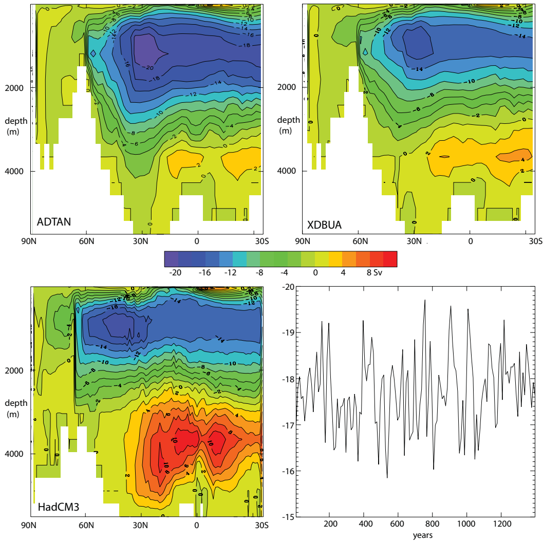
Fig. 13. Atlantic MOC (Sv, clockwise rotation is positive). Top left: average of 100 years from ADTAN; top right: Average of 1400 years from XDBUA; bottom left: climatological average from HadCM3; bottom right: Timeseries of decadal means in XDBUA.
