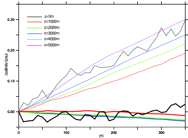
Fig. 3. Global average salinity drifts in FAMOUS. Thin lines are from ADTAN, thick lines are from XDBUA, with both the freshwater drift adjustment and the iceberg calving fluxes applied. The downward trend in salinity in XDBUA comes from an overestimation of the iceberg flux in this run.
