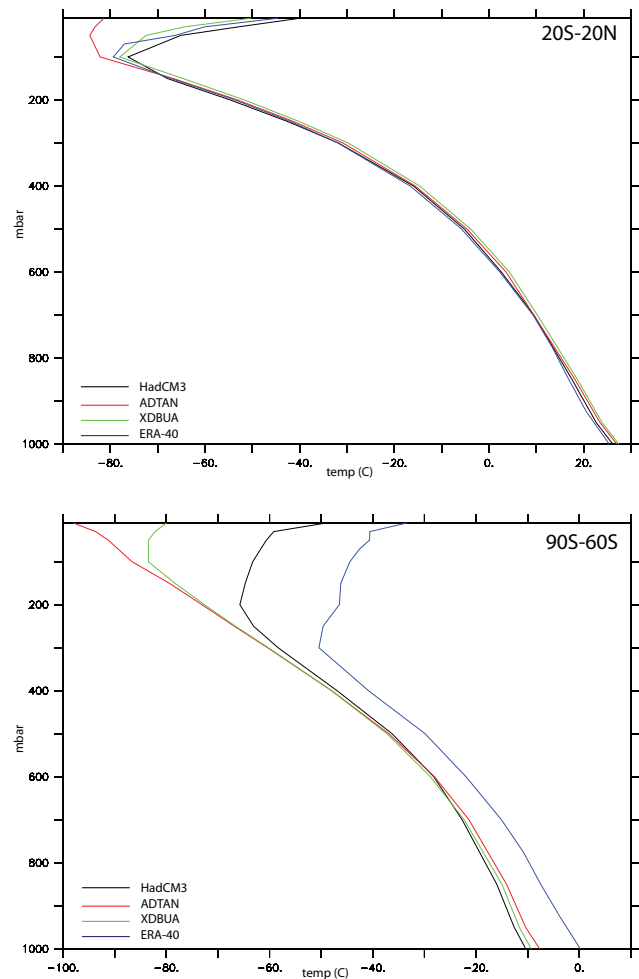
Fig. 5. Horizontally averaged vertical temperature profiles ( ^{\circ}\text{C} ); above: 20^{\circ}\text{S} – 20^{\circ}\text{N} ; below: 90^{\circ}\text{S} – 60^{\circ}\text{S} . ERA-40 climatological data comes from Uppala et al. (2005).
