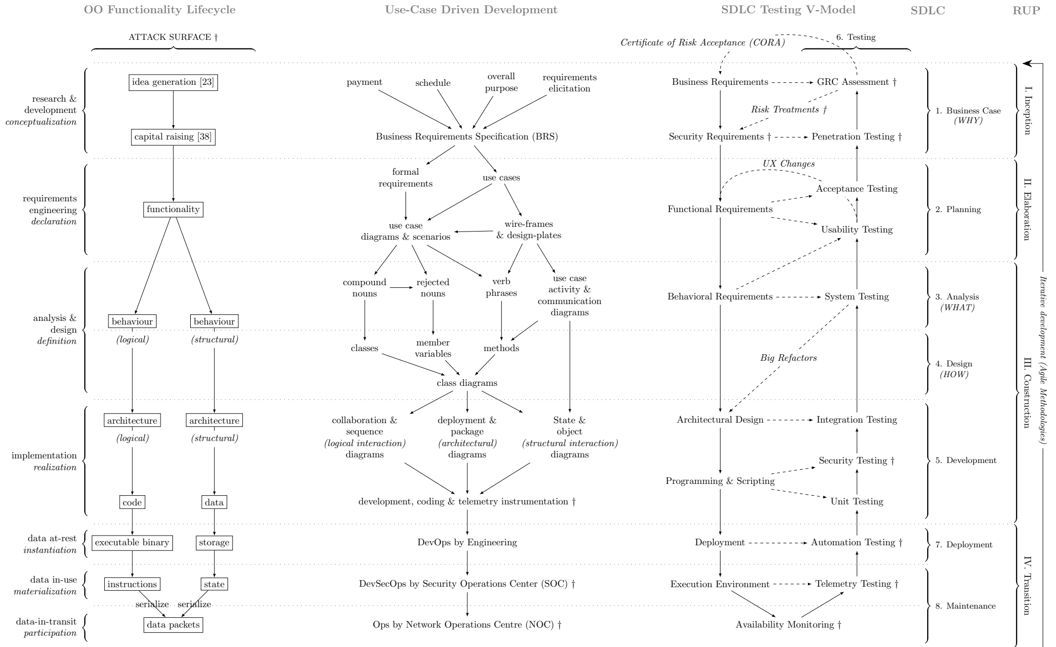
Figure 9: The Software Engineering Standard Model (informal diagram). Vertices marked with † is an opportunity to incorporate information security into the SDLC. Dashed directed edges are test plans unless noted otherwise. (C) COPYRIGHT 2023, Andrew Prendergast. All Rights Reserved.
