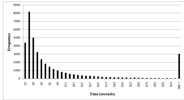
Figure 5: Elapsed times between consecutive submission pairs
