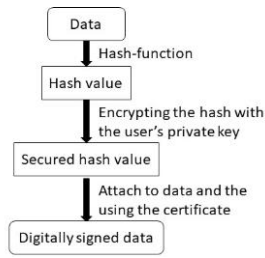
Fig. 2. The signing process in the Blockchain
