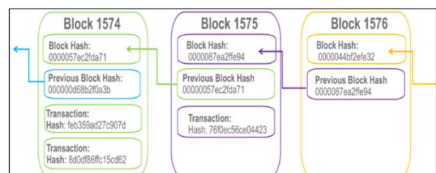
Fig. 1. The sequence of the hash value in the Blockchain [33]
