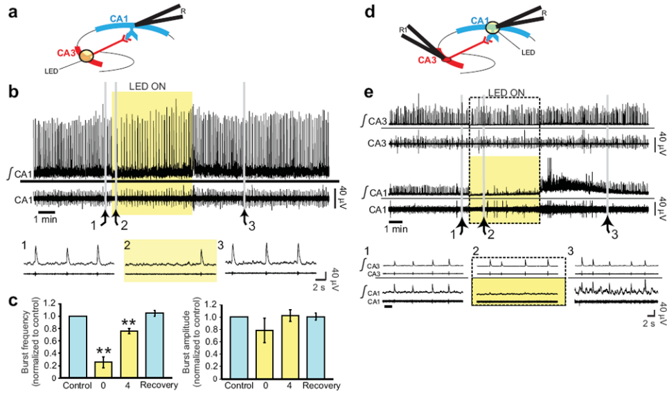
Figure 5. Effective silencing of induced population bursting in the hippocampal circuit in Emx1-Cre;Ai35 mice. (a) Schematic for the inhibition of presynaptic neurons in the hippocampal circuit. K^+ (8 mM) induced population bursting in CA1 was recorded with an extracellular electrode (R). A white light source (LED, yellow circle) was positioned over CA3 to activate Arch-ER2 in presynaptic neurons. (b) Representative traces of the integrated (top) and raw (bottom) population bursting activity from CA1 before (expanded traces in inset 1), during (2), and following (3) the illumination of CA3. Raw population bursting activity is the direct measure of unit activity. Integrated population activity represents the change of unit activity (time constant = 200 ms). (c) Quantified response of population bursting from CA1 ( n = 4 experiments) during 4 intervals: light-off control; the first (0) and final (4) minute of a 5-min exposure to white light; and 5 minutes after light exposure (recovery). Values were normalized to light-off control (** p < 0.01 , repeated measures ANOVA; mean \pm s.e.m.). (d) Schematic for the inhibition of postsynaptic neurons in the hippocampal circuit. Neurons were recorded simultaneously using dual extracellular electrodes (CA1: R, CA3: R1). A white LED was positioned over CA1 to activate Arch-ER2 in postsynaptic neurons. (e) Representative traces of the integrated (top) and raw (bottom) population bursting activity from CA3 and CA1 before (inset 1), during (2), and following (3) illumination to CA1. Light to CA1 led to suppressed bursting from that region, but bursting activity in CA3 was unaffected.
