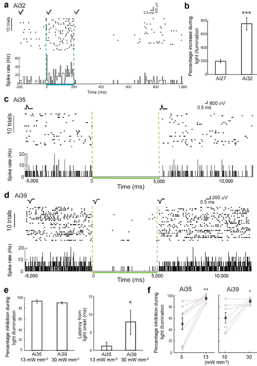
Figure 6. Optical activation or silencing of pyramidal neuron activities in the neocortex of awake Emx1 -Cre;Ai27, Emx1 -Cre;Ai32, Emx1 -Cre;Ai35 and Camk2a -CreERT2;Ai39 mice (abbreviated as Ai27, Ai32, Ai35 or Ai39, respectively, here). (a) Neural activity and spike waveforms in a representative Ai32 neuron before, during and after 200-ms blue light illumination (3 mW mm -2 ). Top, spike raster plot; bottom, histogram of instantaneous firing rate averaged across trials (bin size, 5 ms). (b) Average changes in firing rates upon blue light illumination in Ai27 and Ai32 mice. (***) p < 0.001 (c) Neural activity and spike waveforms in a representative Ai35 neuron before, during and after 5-s green light illumination (13 mW mm -2 ). (d) Neural activity and spike waveforms in a representative Ai39 neuron before, during and after 5-s green light illumination (30 mW mm -2 ). For c and d , top, spike raster plot; bottom, histogram of instantaneous firing rate averaged across trials
