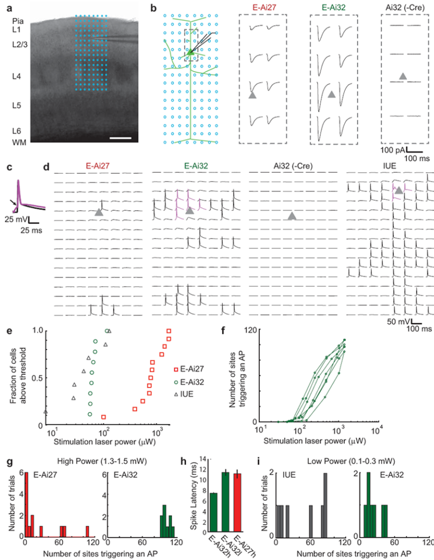
Figure 2. Photostimulation of pyramidal neurons in cortical slices of Emx1-Cre;Ai27 (abbreviated as E-Ai27), Emx1-Cre;Ai32 (E-Ai32), and Ai32 alone (-Cre) mice. (a) A barrel cortex slice with the 8 \times 16 photostimulation grid overlaid (blue dots; spacing 50 \mu\text{m} ). Scale bar, 200 \mu\text{m} . (b) Schematic of the photostimulation geometry and example traces. Whole-cell voltage-clamp traces from the dashed box area (left) are shown for E-Ai27 (with 840 \mu\text{W} light), E-Ai32 ( 70 \mu\text{W} ) and Ai32 ( 1490 \mu\text{W} ). Triangles, soma locations. (c) Waveforms of APs evoked by photoactivating the somata and dendrites (magenta) and axons (black). The arrow marks the inflection point. (d) Whole-cell current-clamp traces showing evoked APs in the 8 \times 16 grid for a typical cell each of E-Ai27 ( 1700 \mu\text{W} ), E-Ai32 ( 155 \mu\text{W} ), Ai32 ( 1500 \mu\text{W} ), and IUE ( 155 \mu\text{W} ). (e) Minimum laser power required to evoke an AP from at least one stimulation site. (f) Number of photostimulation sites evoking an AP as a function of laser power in E-Ai32 neurons ( n = 7 ). (g) Number of stimulation sites triggering APs using high laser powers. (h) Spike latencies of somatic/dendritic APs from the light onset. E-Ai32h: E-Ai32 cells ( n = 9 cells, 143 APs) under high powers ( > 1 \text{ mW} ). E-Ai32l: E-Ai32 cells ( n = 9 cells, 28 APs) under low powers ( < 100 \mu\text{W} ). E-Ai27: E-Ai27 cells ( n = 2 cells,
