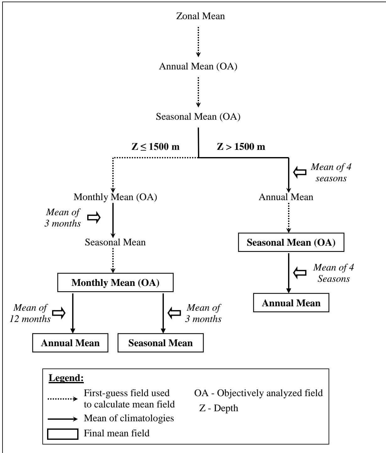
Figure 2. Scheme used in computing annual, seasonal, and monthly objectively analyzed means for dissolved oxygen ( O_2 ), Apparent Oxygen Utilization (AOU), and oxygen saturation ( O_2^S ).
