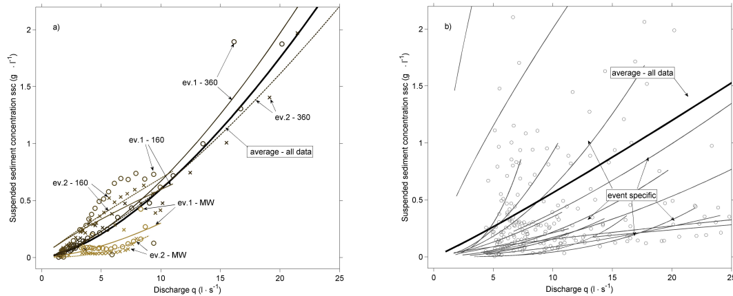
Fig. 10. Relationship between sediment concentrations and discharge of the flooding experiments (a) and natural events (b), modified from Eder et al., 2010) in the HOAL catchment.
