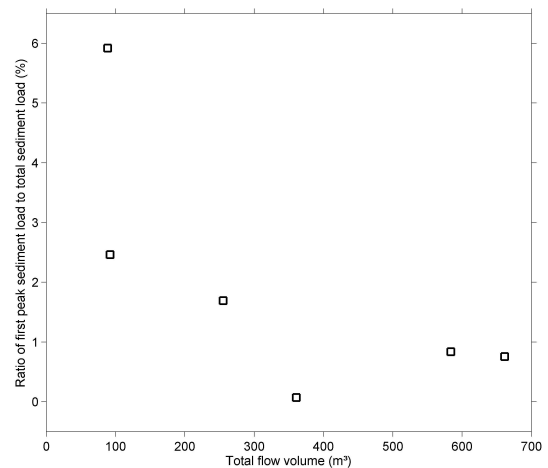
Fig. 11. Ratio of first flush sediment load to total sediment load of natural events as a function of total flow volume in the in the HOAL catchment (64 ha) (see Table 3).
