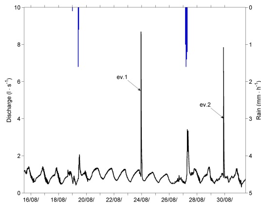
Fig. 5. Hyetograph and discharge at the catchment outlet (site MW) 10 days before and during the flooding events in August 2011.
