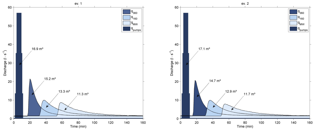
Fig. 6. Hydrographs of the first (ev.1) and second (ev.2) flooding experiment at the flood initiation location and three monitoring sites (see Fig. 2).
