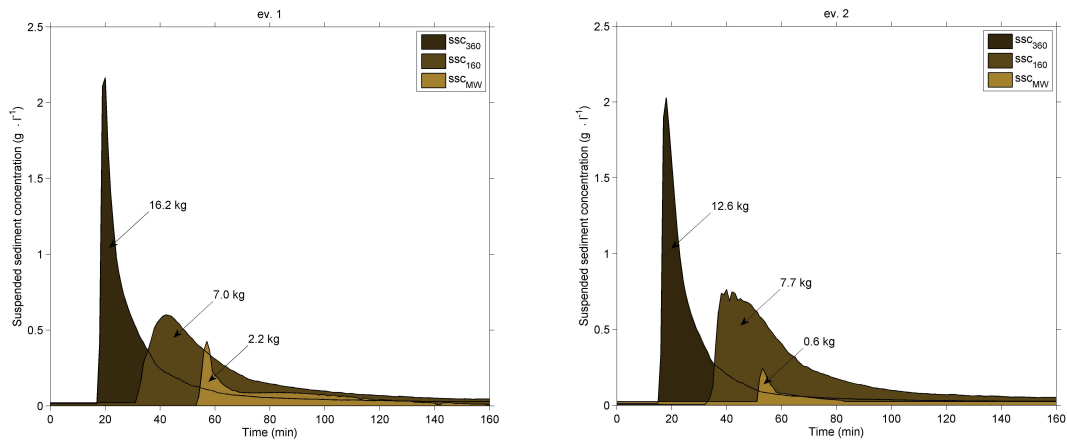
Fig. 7. Sedigraphs of the first (ev.1) and second (ev.2) flooding experiments at the three monitoring locations (see Fig. 2).
