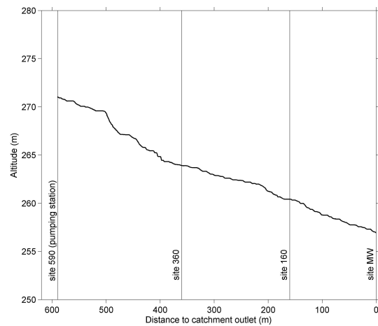
Fig. 3. Longitudinal section of the stream in the HOAL catchment with measurement sites.
