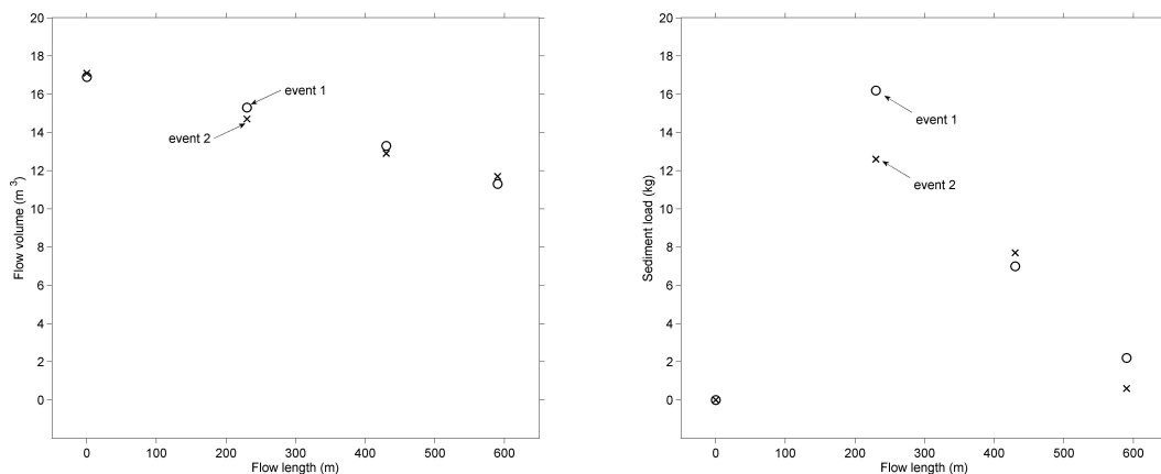
Fig. 8. Comparison of water volumes and sediment loads transported along the stream for the two flooding experiments (event 1 and event 2). Water flow is from left to right.
