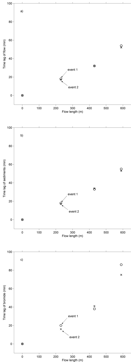
Fig. 9. Time lag of water (celerity) (a), sediment (b) and bromide (velocity) (c) for the two flooding experiments (event 1 and event 2) estimated from the first appearance (first rise) of the signal.
