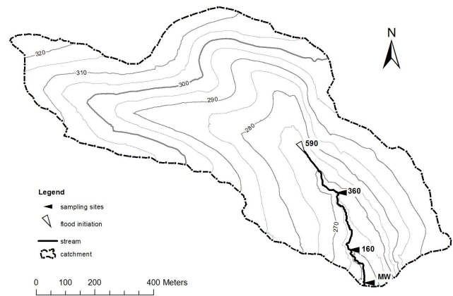
Fig. 2. HOAL catchment with point of flood initiation (590) and measurement sites (360, 160, MW).
