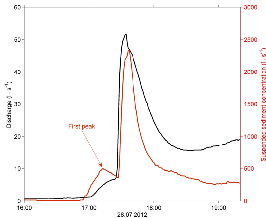
Fig. 1. Natural event with single peaking hydrograph and double peaking sedigraph in the HOAL Petzenkirchen catchment (0.64 ha) on 28 July 2012.
