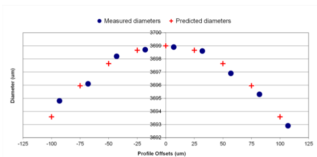
Figure 3. Diameter measurements (solid circle) from nine parallel traces at 25 μm increments through the central region of the Brinell indentation. Also shown are predicted diameter values (cross) based on a circular indentation.
