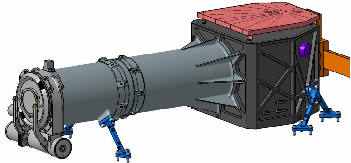
Figure 7. Coronagraph COB overview.
