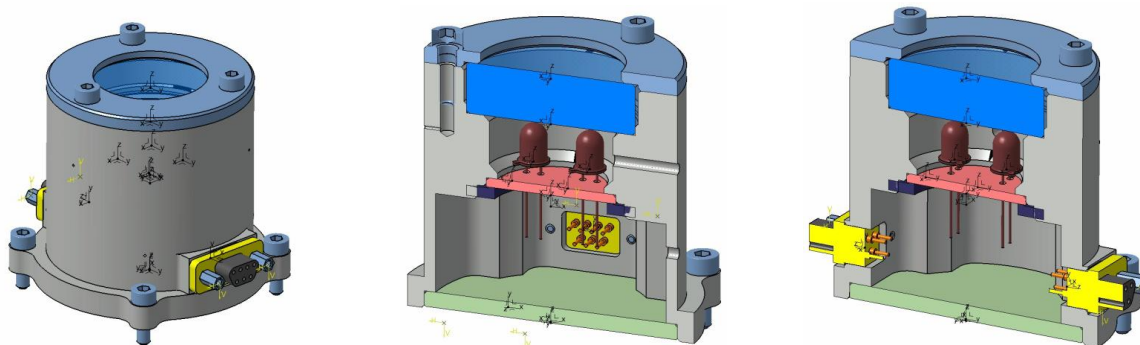
Figure 13. Occluder position sensor emitter head (OPSE), preliminary design reproduced from Phase-B Design Report, courtesy of LAM.
