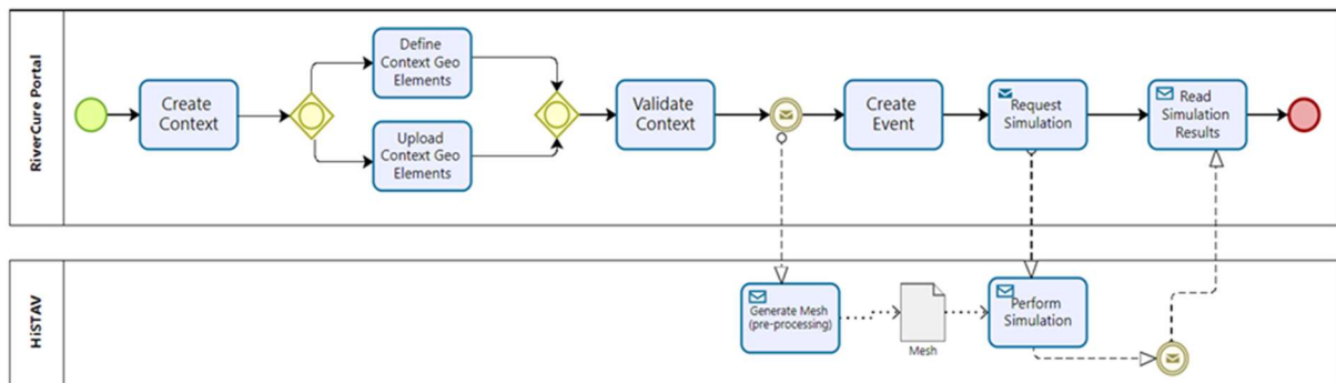
Figure 18 - Activities diagram of Context creation (in BPMN)
