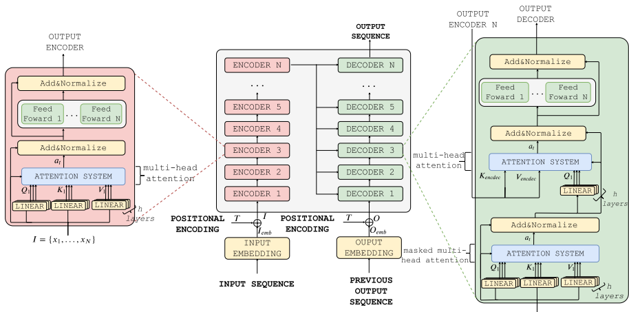
Fig. 19 Illustration of Neural Transformer (Vaswani et al. 2017) for machine translation. The architecture consists of several stacked attentional encoders and decoders. The encoder process is massively parallel and eliminates recurrences, and the decoder generates the translated words sequentially. Each encoder uses multiple heads of the self-attention mechanism followed by fusion and normalization layers. Similarly, to generate the output, each decoder has multiple heads of self-attention and masked-self attention to mask words not yet generated
