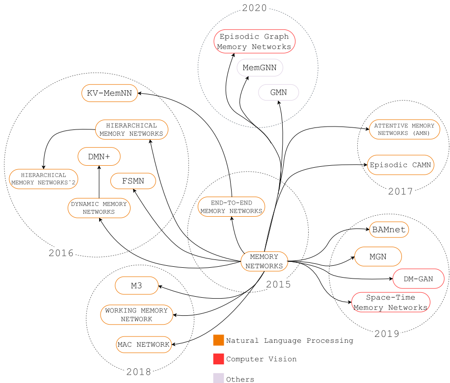
Fig. 5 Memory-based neural networks (MemNN). Architectures labels are color-coded as follows: orange—natural language processing, red—computer vision, purple—others. The end-to-End Memory networks is the first end-to-end differentiable version of MemNN. GMN (Ahmadi et al. 2020) and MemGNN (Ahmadi et al. 2020) are the first graph networks with memory. DMN (Xiong et al. 2016), MemGNN (Ahmadi et al. 2020), Episodic graph memory networks (Lu et al. 2020), Episodic CAMN (Abdulnabi et al. 2017), are the first instances of the episodic memory framework. (Color figure online)
