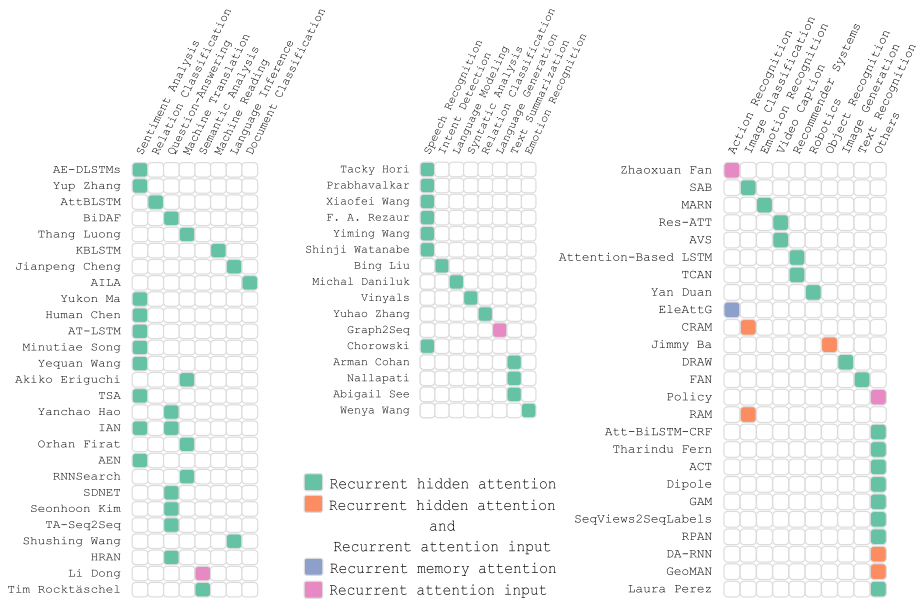
Fig. 14 Attention-based recurrent neural networks main architectures by task and attention use
