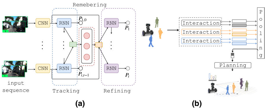
Fig. 23 Illustration of deep visual odometry with Adaptive Memory (Xue et al. 2020) and Crowd-Robot Interaction (Chen et al. 2019a) for navigation. a The deep visual odometry with adaptive memory framework. This framework introduces two important components called remembering and refining , as opposed to classic frameworks that treat VO as just a tracking task. Remembering preserves long-time information by adopting an adaptive context selection, and refining improves previous outputs using spatial-temporal feature reorganization mechanism. b Crowd–Robot Interaction network. The network consists of three modules: interaction, pooling, and planning. Interaction extracts robot–human interactions in crowds. Pooling aggregates all interaction information, and planning estimates the state’s value based on robots and humans for navigation in crowds
