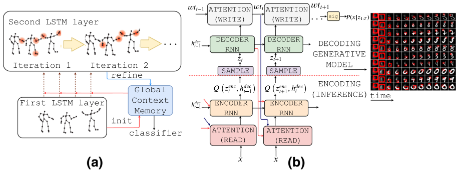
Fig. 20 Illustration of global context-aware attention (Liu et al. 2017c) for action recognition, and DRAW (Gregor et al. 2015) for image generation. a The Context-Aware Attention Network. The first LSTM layer encodes the skeleton sequence and generates an initial global context memory. The second layer performs attention over the inputs with global context memory assistance and generates a refined representation. The refine representation is then used back to the global context. Multiple attention iterations are carried out to refine the global context progressively. Finally, memory information is used for classification. b The DRAW architecture. At each time step t , the input is read by attention and passed to the encoder RNN. The encoder's output is used to compute the approximate posterior over the latent variables. On the right, an illustration shows the iterative process of generating some images. Each row shows successive stages in the generation of a single digit. The network guided by attention draws and refine regions successively. The red rectangle delimits the area attended to by the network at each time-step
