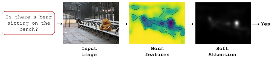
Fig. 8 An intuitive example of soft attention. Visual QA architecture outputs an answer given an image and a textual question as input. It uses a soft attention mechanism that weighted visual features for the task for further processing. The premise is that the norm of the visual features correlates with their relevance. Besides, those feature vectors with high magnitudes correspond to image regions that contain relevant semantic content
