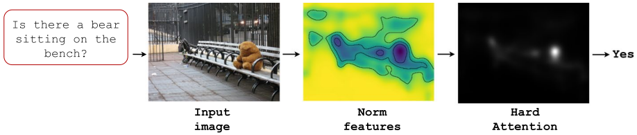
Fig. 9 An intuitive example of hard attention. Given an image and a textual question as input, the Visual QA architecture outputs an answer. It uses a hard attention mechanism that selects only the important visual features for the task for further processing
