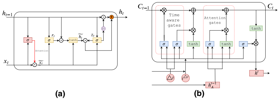
Fig. 15 Recurrent memory attention approaches. a Illustration of Element-wise-attention gate in GRU. Specifically, the input modulation is adaptable to the content and is performed in fine granularity, element-wise rather than input-wise. b Gate attention in LSTM. The model calculates attention scores to weigh the relevance of different parts of history. There are two additional gates for updating the current cell using the previous state h_{t-1}^A . The first, input attention gate layer, analyzes the current input i^{\Delta t} and h_{t-1}^A to determine which values to be updated in current cell C^t . The second, the modulation attention gate, analyzes the current input i^{\Delta t} and h_{t-1}^A . Then computes the set of candidate values that must be added when updating the current cell state C^t . The attention mechanisms in the memory cell help to more easily capture long-term dependencies and the problem of data scarcity
