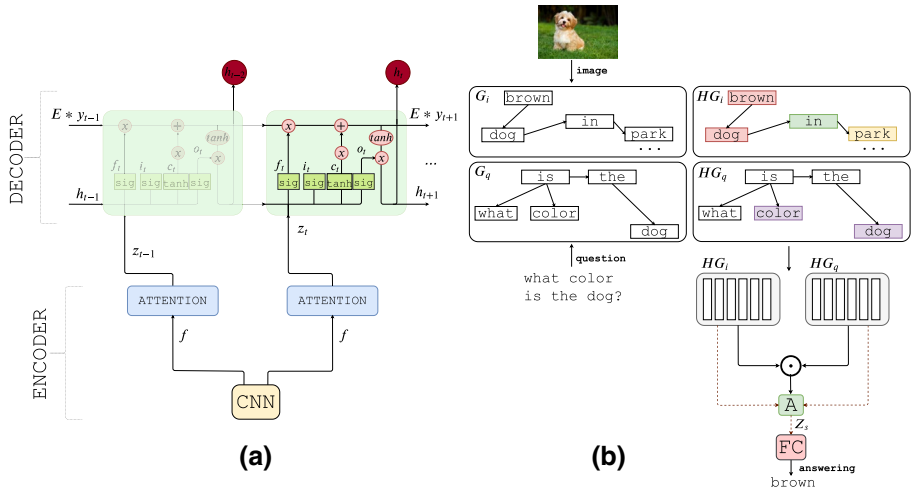
Fig. 21 Illustration of classic attentive encoder–decoder framework by Xu et al. (2015) and Hypergraph Attention Network (Kim et al. 2020a) for question answering tasks. a The show, attend and tell framework. At each time step t , attention takes as input visual feature maps and previous hidden state of the decoder and produces a dynamic context vector with essential visual features to predict the next word. b The Hypergraph Attention Network. For a given pair of images and questions, two symbolic graphs G_i , and G_q are constructed. After, two hypergraphs HG_i , and HG_q with random-walk hyperedge are constructed and combined via co-attention map A . Finally, the final representation Z_s is used to predict an answer for the given question
