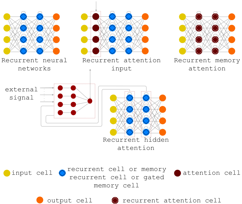
Fig. 13 Attention-based recurrent neural networks. The architecture is a classic recurrent network or a Bi-RNN when hidden layers are recurrent cells. When the hidden layer is a recurrent memory, the architecture is an LSTM or Bi-LSTM. Finally, the architecture is a GRU when the hidden layer is a gated memory cell. The recurrent attention input group uses attention to filter input data. Recurrent hidden attention groups automatically select relevant encoder hidden states across all time steps. Usually, this group implements attention in encoder–decoder frameworks. The recurrent memory attention group implements attention within the memory cell. There are not many architectures in this category as far as we know, but the main uses are related to filtering the input data and the weighting of different historical components for predicting the current time step
