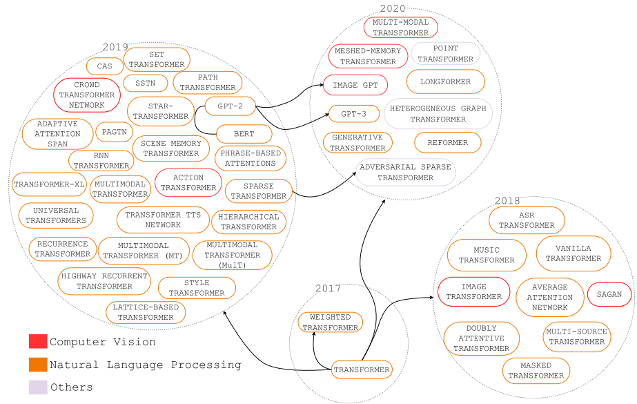
Fig. 6 Transformer-based neural networks. Architectures labels are color-coded as follows: orange—natural language processing, red—computer vision, purple—others. (Color figure online)
