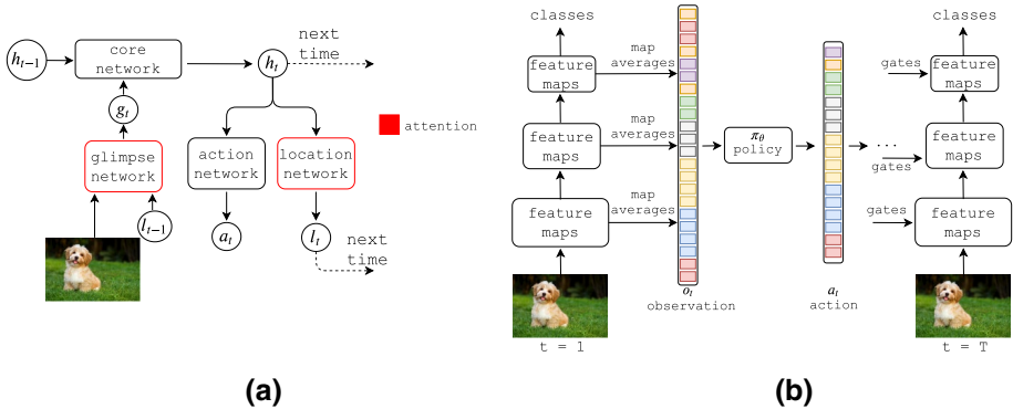
Fig. 22 Illustration of RAM (Mnih et al. 2014) and dasNet (Stollenga et al. 2014) for image classification tasks. a The RAM framework. At each time step t , the glimpse networks extracts a retina-like representation based on input image and an focus location l_{t-1} . The core network takes the glimpse representation as input and combining it with the internal representation at the previous time step and produces the new internal state of the model h_t . The location network and action network use the h_t to produce the next location l_t to attend and the classification. b The dasNet network. Each image is classified after T passes through CNNs. After each forward propagation, the averages of feature maps are combined into an observation vector o_t , that is used by a deterministic policy to choose an action a_t that changes the focus of all the feature maps for the next pass of the same image. Finally, after pass T times, the output is used to classify the image
