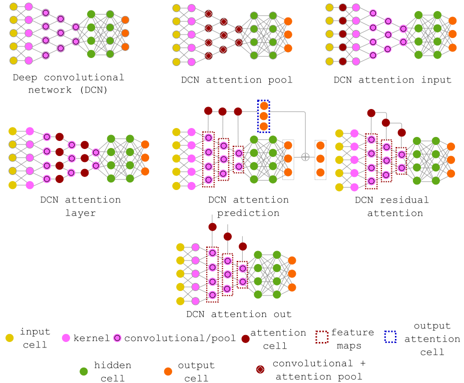
Fig. 11 Attention-based convolutional neural networks. DCN attention pool group uses an attention pool, instead of regular pooling, as a strategy to determine the importance of each individual in a given feature map window. The premise is that only a few of these windows are significant and must be selected concerning a particular objective. DCN attention input group uses structures similar to the human's visual attention. DCN attention layer group collects important stimuli of high (semantic level) and low level (saliency) for subsequent layers of architecture. DCN attention prediction group uses attention in the final stages of prediction, sometimes as an ensemble element. DCN residual attention group uses attention as a residual module between any convolutional layers to mitigate the vanishing problem, capturing only the relevant stimuli from each feature map. DCN attention out-group can represent the category of recurrent attention processes
