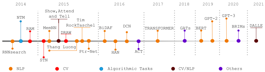
Fig. 7 Key developments in attention in DL timeline. RNNSearch presented the first attention mechanism. NTM and Memory networks introduced memory and dynamic flow control. RAM and DRAW learned to combine multi-glimpse, visual attention, and sequential processing. STN introduced a module to increase the robustness of CNNs to variations in spatial transformations. Show, attend and tell created attention for multimodality. The Ptr-Net used attention as a pointer. BiDAF, HAN, and Dynamic Coattention Network (DCN) presented attentional techniques to align data with different hierarchical levels. ACT introduced the computation time topic. Transformer (Vaswani et al. 2017) was the first self-attentive neural network with an end-to-end attention approach. GATs introduced attention in GNNs. BERT (Devlin et al. 2019), GPT-2 (Radford et al. 2019), GPT-3 (Brown et al. 2020), and DALL-E are the state-of-the-art in language models and text-to-image generation. Finally, BRIMs (Mittal et al. 2020) learned to combine bottom-up and top-down signals
