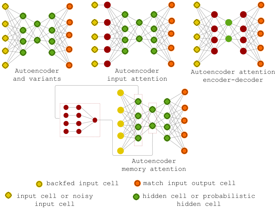
Fig. 16 Attention-based generative models. The Autoencoder input attention group uses attention to facilitate the decomposition of scenes in abstract building blocks. The input components extracted by the masks share significant properties and help to imagine new scenarios. This approach is very efficient for the network to learn to decompose challenging scenarios between semantically significant components. Autoencoder memory attention group handles a memory buffer that allows read/writes operations and is persistent over time. Such models generally handle input and output to the memory buffer using write/read operations guided by the attention system. The use of attention and memory history in autoencoders helps to increase the generalizability of architecture. Autoencoder attention encoder–decoder using a model (usually self-attentive model) to increase the ability to generalize
