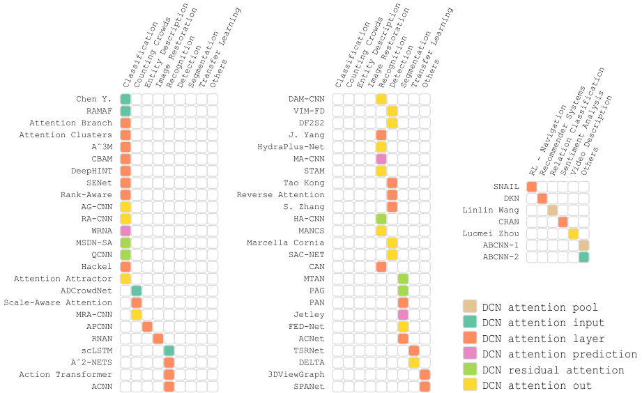
Fig. 12 Attention-based convolutional neural networks main architectures by task and attention use
