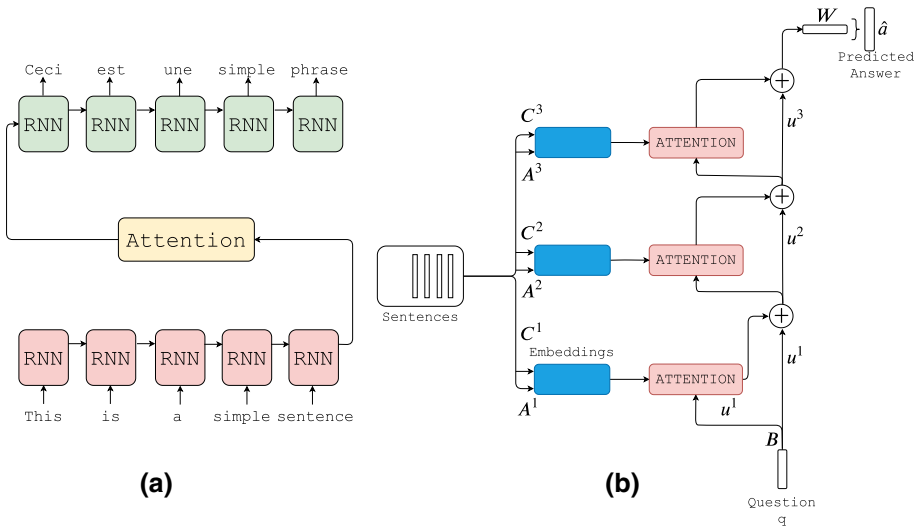
Fig. 18 Illustration of RNNSearch (Bahdanau et al. 2015) for machine translation, and End-to-End Memory Networks (Sukhbaatar et al. 2015) for question answering. a The RNNSearch architecture. The attention guided by the decoder’s previous state dynamically searches for important source words for the next time step. b The End-to-End Memory Networks. The architecture consists of external memory and several stacked attention layers modules. To generate a response, the model makes several hops in memory using only attentional layers
