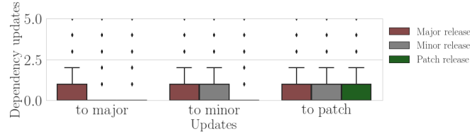
Fig. 4: Number of updated dependencies between package releases, classified by release type of the update.
