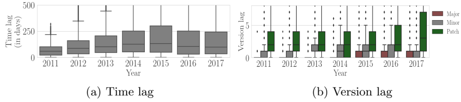
Fig. 8: Distribution of technical lag, per year, in outdated dependencies.
