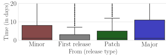
Fig. 10: Time required to update a package release to a more recent patch.
