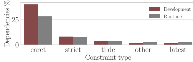
Fig. 2: Proportion of the types of dependency constraints used in npm.
