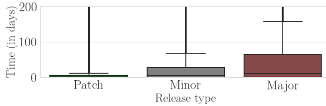
Fig. 6: Time needed to update a package to a patch, minor or major release.
