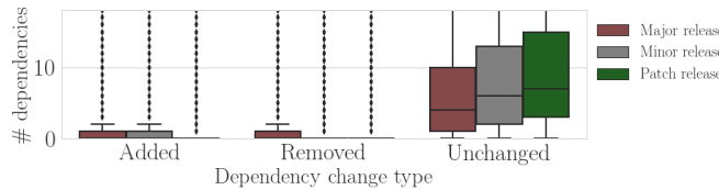
Fig. 3: Number of removed, unchanged and added dependencies between subsequent package releases
