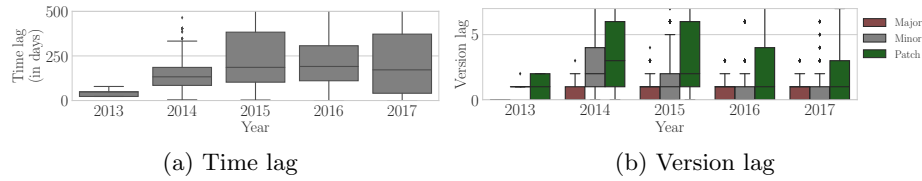
Fig. 1: Time and version lag distribution, per year, for all outdated dependencies of eslint .
