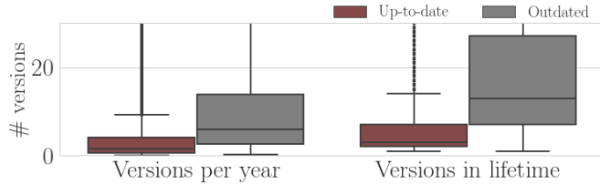
Fig. 9: Number of available versions of packages used by outdated and up-to-date dependencies.
