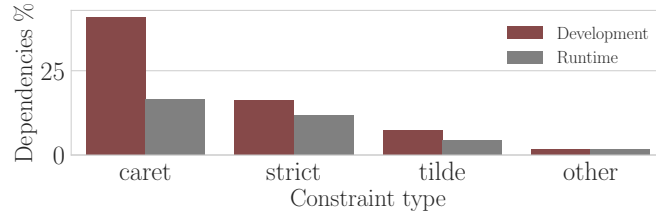
Fig. 7: Proportion of the types of constraints used for outdated dependencies.
