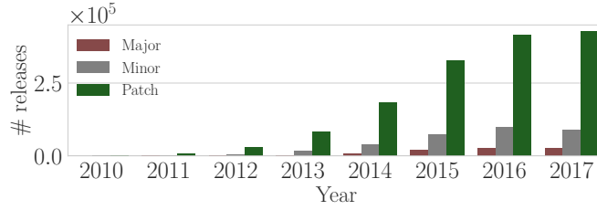
Fig. 5: Number of releases of required packages in npm , per year and per release type.
