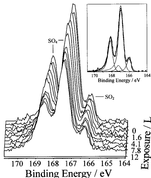
FIG. 7. S 2 p fast XP spectra during C 2 H 4 adsorption over sulphated Pt{111} at 95 K. \theta(\text{SO}_4) = 0.25 ML. Inset shows spectral deconvolution.
