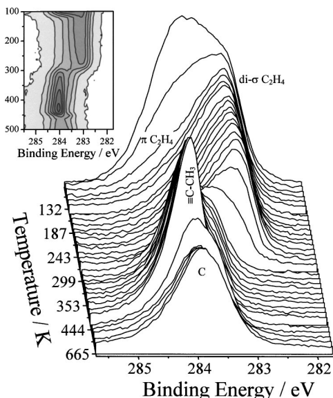
FIG. 9. C 1s fast XP temperature programmed reaction spectra from a saturation C_2H_4 adlayer on SO_4 -precovered Pt{111}. Inset shows corresponding image plot.
