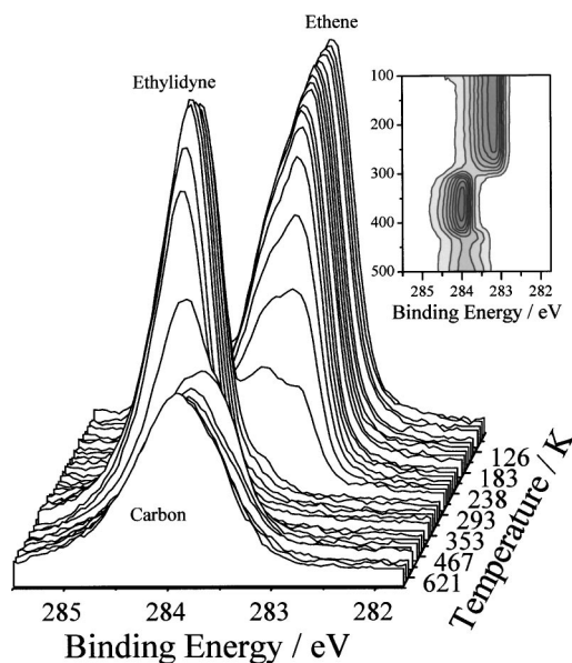
FIG. 2. C 1s fast XP temperature programmed reaction spectra from a saturation C_2H_4 adlayer on clean Pt{111}. Inset shows corresponding image plot.
