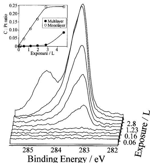
FIG. 1. C 1s fast XP spectra during C_2H_4 adsorption on clean Pt{111} at 95 K. Inset shows fitted component intensities.
