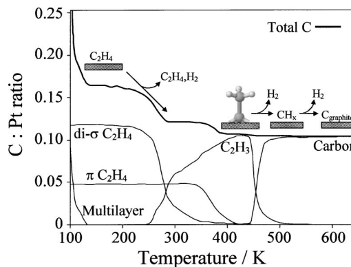
FIG. 10. Fitted C 1s intensities as a function of temperature for a saturation C_2H_4 adlayer on SO_4 -precovered Pt{111}. The total integrated C signal is also shown.
