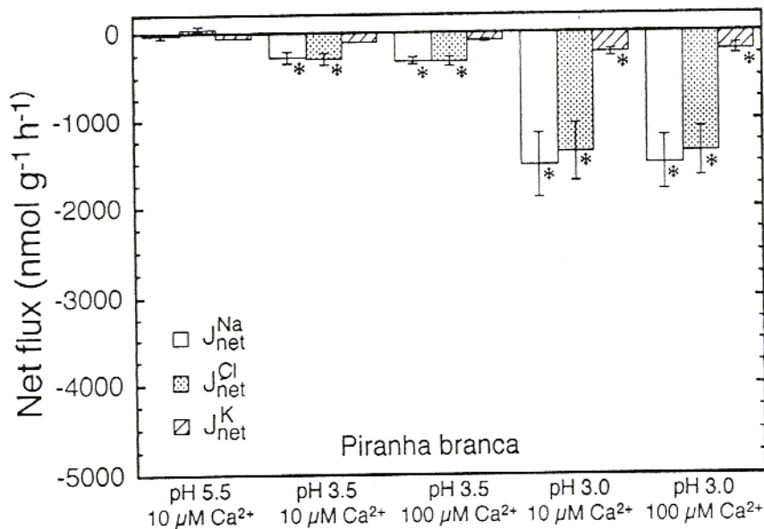
Figure 4. Effects of water pH and Ca^{2+} concentration on net Na^+ flux ( J_{net}^{Na} ), net Cl^- flux ( J_{net}^{Cl} ), and net K^+ flux ( J_{net}^{K} ) of piranha branca ( Serrasalmus cf. holandi ) from the Rio Negro. Fluxes were measured during the first hour of exposure to each low pH. Values are means \pm SE. The y-axis is drawn with the same scale as Figure 1 to facilitate comparisons. Asterisks indicate significant differences from corresponding fluxes at pH 5.5.
