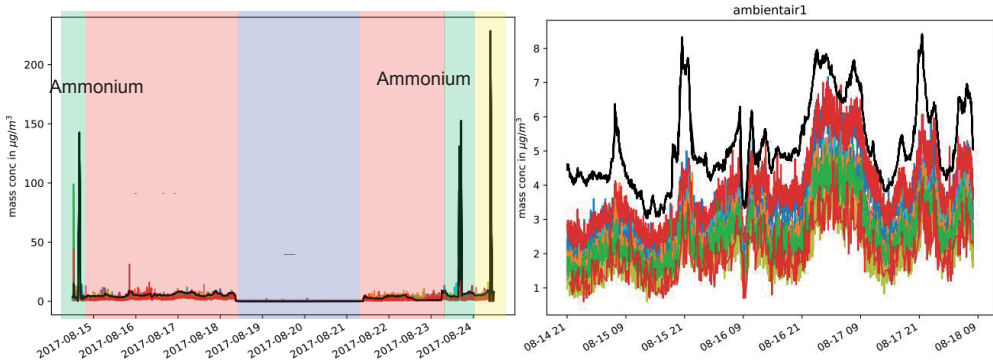
Fig. 4. Time series of experiments with different polydisperse aerosols (left) and zoomed in for PM 2.5 mass for the first session of ambient air measurements (right). The reference is the solid black line
