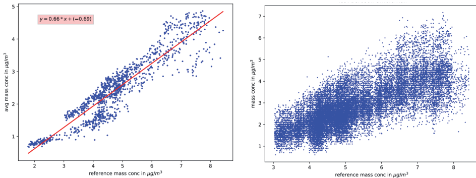
Fig. 5. Scatterplots: mean PM 2.5 mass against the reference (left) and for all individual 14 valid sensors for the test aerosol ambient air (right).
