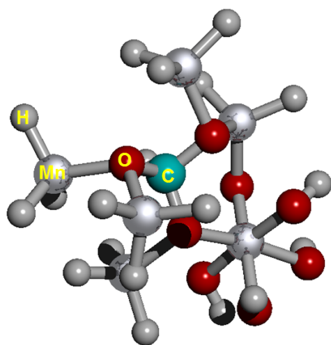
Figure 2. Cell structure of a protonated rhodochrosite crystal. Represented in red the oxygen; silver in color Manganese; in gray color Hydrogen; in light see green color the Carbon. Stoichiometry: \text{CMn}_6\text{O}_8 . Stoichiometry protonated: \text{CH}_{19}\text{Mn}_6\text{O}_8
