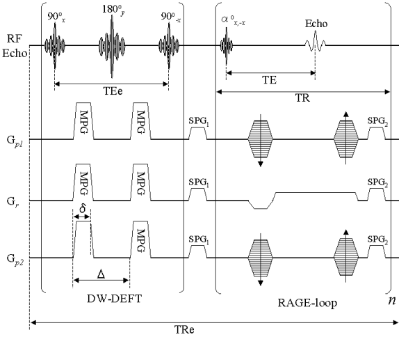
Fig. 1. Diagram of the 3D MP-RAGE MRI pulse sequence used for 3D diffusion mapping (3D-DWI). The slice phase-encode gradient ( G_{p1} -PEG) happens only once per TR_e period. On the other hand, the phase-encode gradient ( G_{p2} -PEG) changed in each TR period. In order to avoid T1-contamination in the DW image, the phase encoding was centric k-space acquisition order.
