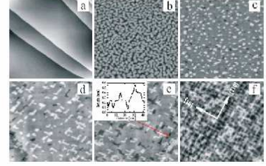
Figure 2: STM images for (a) clean Pd(100) substrate ( 500 \times 500 \text{ nm}^2 ); (b) 0.85 ML Cu ( 100 \times 100 \text{ nm}^2 ); (c) 2.1 ML Cu ( 100 \times 100 \text{ nm}^2 ); (d) 3.05 ML Cu ( 100 \times 100 \text{ nm}^2 ); (e) 6.0 ML Cu ( 100 \times 100 \text{ nm}^2 ); (f) 9.0 ML Cu ( 100 \times 100 \text{ nm}^2 ) deposited at 300 K.
