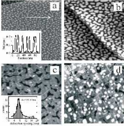
Figure 1: STM images for (a) 0.5 ML Pd ( 200 \times 200 \text{ nm}^2 ); (b) 1.6 ML Pd ( 200 \times 200 \text{ nm}^2 ); (c) 4.8 ML Pd ( 100 \times 100 \text{ nm}^2 ); (d) 6.0 ML Pd ( 100 \times 100 \text{ nm}^2 ) deposited at 300 K.
