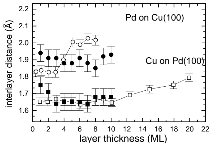
Figure 3: Perpendicular interlayer distance calculated based on a kinetic model from LEED intensity of the (00) diffraction beam vs. energy curves. The change of the interlayer distance occurs at about 3–4 ML for Pd/Cu(100) films and at about 10 ML for Cu/Pd(100) films. Assuming a pseudomorphic growth up to 3 ML for Pd on Cu(100) and 10 ML for Cu on Pd(100), PLD films can be identified as fcc Pd and fct Cu structures. The results from experimental and theoretical work at 300 K are indicated by open and solid symbols, respectively. The lines are guides to eye.
