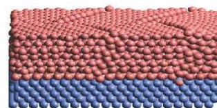
Figure 5: Typical configuration of stacking faults for 7 ML Pd on Cu(100) based on molecular dynamics annealing. The lateral size is 20 \times 20 atom 2 . The misfit dislocations orientate along the \langle 100 \rangle direction of the substrate.
