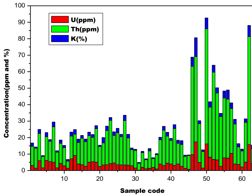
Fig. 4: The ^{238}\text{U} , ^{232}\text{Th} and ^{40}\text{K} Content.
