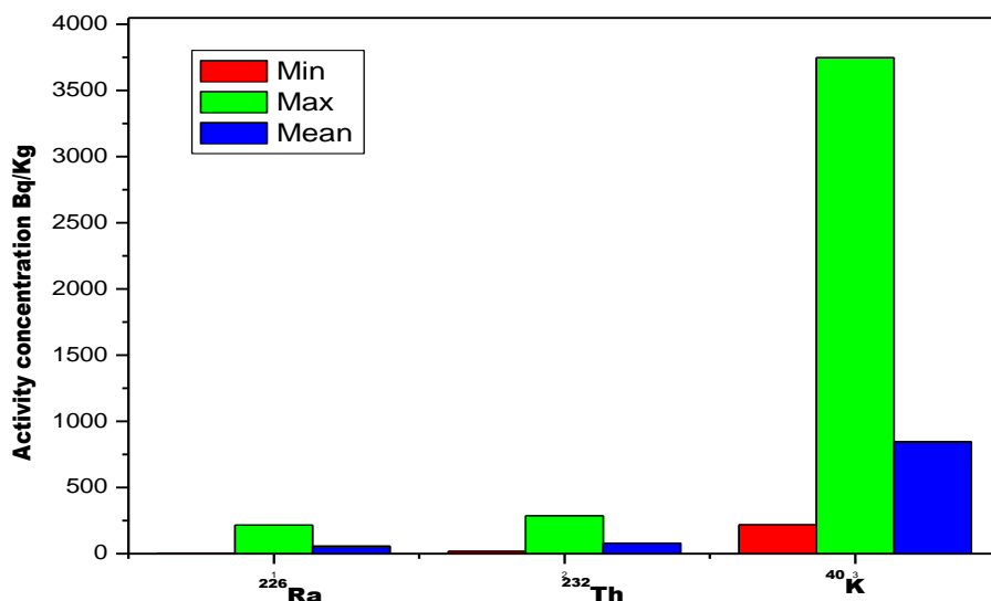
Fig.3: Activity concentration in (Bq/Kg) of ( 226 Ra), 232 Th and 40 K
