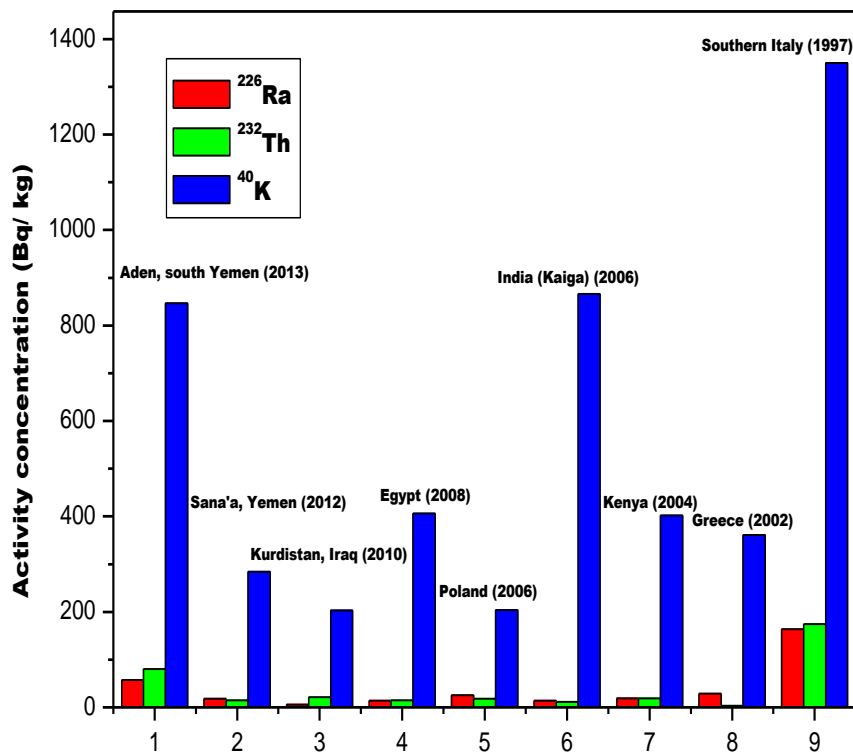
Fig. 5: Comparison of the resulted activity concentration with those of other countries.
