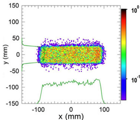
Figure 7. Beam density in real space at the lithium target footprint of 200\text{ mm} \times 50\text{ mm} . The density profile projected on both axes is also shown [44].
