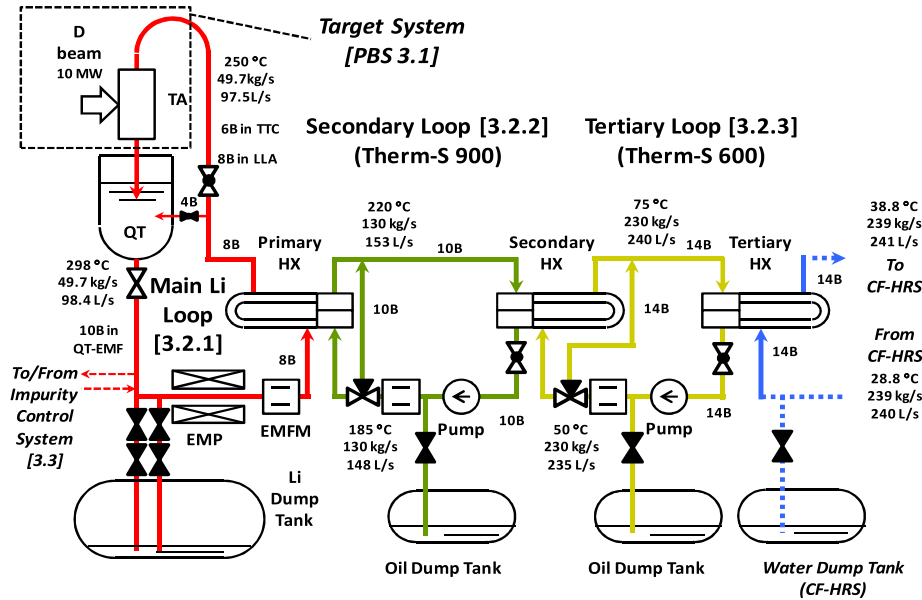
Figure 11. Block flow diagram of the heat removal system.
