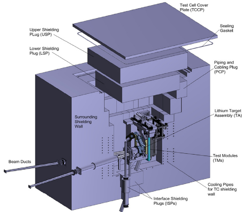
Figure 15. TC with internals and penetrations for beam tubes as well as a lithium loop inlet and outlet pipes.
