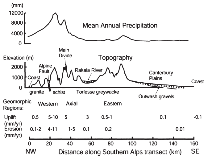
Fig. 2. Cross section through the central Southern Alps, New Zealand, showing mean annual precipitation, uplift and erosion rates. Modified from Whitehouse. 6
