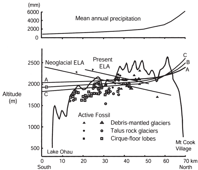
Fig. 5. Profile of the Ben Ohau Range showing the distribution of active and fossil rock glacier sites. Postulated range of the -2^{\circ}\text{C} isotherm indicated by lines A to C. ELA = glacier equilibrium line altitude. Modified from Brazier et al. 10
