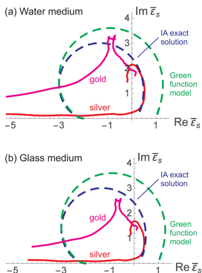
Figure 4. Evolution of the normalized permittivity \bar{\epsilon}_s = \epsilon_s/\epsilon_b in the complex plane as the vacuum wavelength is varied for silver nanoparticles (red) \lambda_v \in \{188\text{--}500\} nm and gold nanoparticles (magenta) \lambda_v \in \{188\text{--}600\} nm embedded in a water medium N_b = 1.33 (a), and a glass medium N_b = 1.5 (b). The values of \bar{\epsilon}_s required to reach ideal absorption in the lowest electric dipole mode are plotted in dashed blue for kR varying from 0 to 4. The intersections between this curve and the measured metal permittivity provide the conditions to optimize absorption using silver or gold nanoparticles. Tables 1 and 2 detail these conditions for water and glass media. For comparison, we also represent the Green function point-like predictions of eq 12 in dashed green. As already noted in Figure 1, this model fails in accurately predicting the IA conditions.
