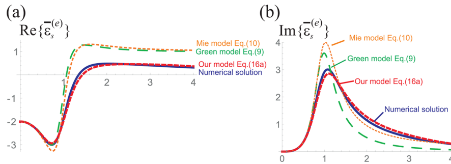
Figure 1. Numerical results of the real and imaginary parts of \bar{\epsilon}_s , yielding the lowest IA solution are plotted as a function of kR (blue solid curves). The predictions from the Green function point-like model eq 9 are plotted in green (long dashed lines), and the Mie theory development model eq 10 are plotted in orange (dotted lines). Our analytical model eq 16a (red short dashed curves) provides an improved description of the conditions to reach ideal absorption over a broad kR range.
