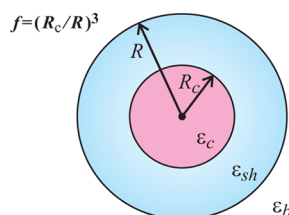
Figure 6. Schematic of a concentric coated sphere where the core, shell, and background permittivities are denoted, respectively, \epsilon_c , \epsilon_{sh} , and \epsilon_b . The filling fraction of the core material is defined as f \equiv (R_c/R)^3 .
