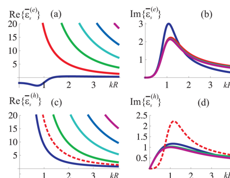
Figure 2. Conditions to reach electric dipole Ideal Absorption as a function of kR for the real (a) and imaginary (b) part of the complex permittivity \bar{\epsilon}_s . Magnetic dipole IA values for \bar{\epsilon}_s are also plotted in (c,d). The lowest electric dipole solution with \mathcal{R}\{\bar{\epsilon}_s\} > 1 is plotted as a dashed curve in (c) and (d) for comparison.
