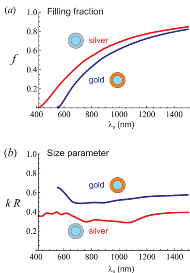
Figure 7. Plots of the filling fraction (a) and the size parameter (b), required to achieve IA in a core-shell structure immersed in a N_b = 1.5 background material. The core is considered to be a lossless high index material, N_c = 2.8 , and the shell is either silver (red line) or gold (blue line).
