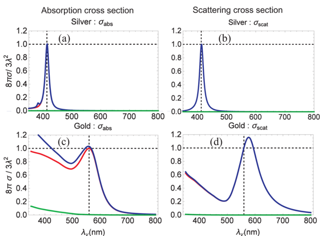
Figure 5. Absorption (a) and scattering (b) cross sections for silver nanoparticles designed to reach IA in glass medium N_b = 1.5 (blue curves). Dipole contributions to the cross sections are plotted in red for the electric dipole and green for the magnetic dipole. The silver nanoparticle diameter is D_{IA} = 30.6 nm. The IA wavelength is specified by a vertical dashed line, and corresponds to the situation of the cross section reaching the limit of eq 6. (c, d) Same as (a, b) for gold nanoparticles of diameter D_{IA} = 76.2 nm.
