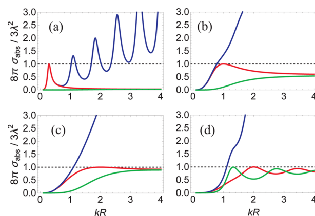
Figure 3. Dimensionless absorption cross sections, 8\pi\sigma_{\text{abs}}/(3\lambda^2) , plotted as a function of kR for IA designed to occur at: (a) kR = 0.3 , \bar{\epsilon}_s = -2.21 + i0.0611 ; (b) kR = 1 , \bar{\epsilon}_s = -1.87 + i2.91 ; (c) kR = 2 , \bar{\epsilon}_s = 0.4809 + i1.148 ; and (d) kR = 2 , \bar{\epsilon}_s = 4.968 + i1.361 . Total absorption cross sections are given by blue curves, electric dipole absorption by red curves, and magnetic dipole absorption by green curves.
