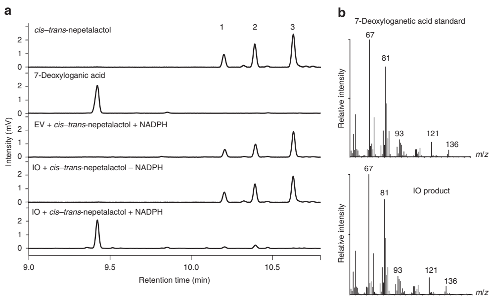
Figure 4 | Functional characterization of IO. The cytochrome P450 enzyme was expressed in yeast and assayed as a microsomal preparation by incubation with cis-trans -nepetalactol and \text{NADPH} . (a) GC-MS profile of the reaction extract compared with the negative control and authentic standards. (b) Product identity was confirmed by comparison of the MS spectrum with the authentic standard. Cis-trans -nepetalactol is the peak 3 (ref. 13), in the substrate standard, peaks 1 and 2 are its open dialdehyde forms ( cis and trans iridodial). These compounds are in equilibrium in water 12 . Peak 3 is the first converted by IO, but eventually, possibly after interconversion, all three compounds are metabolized (not shown).
