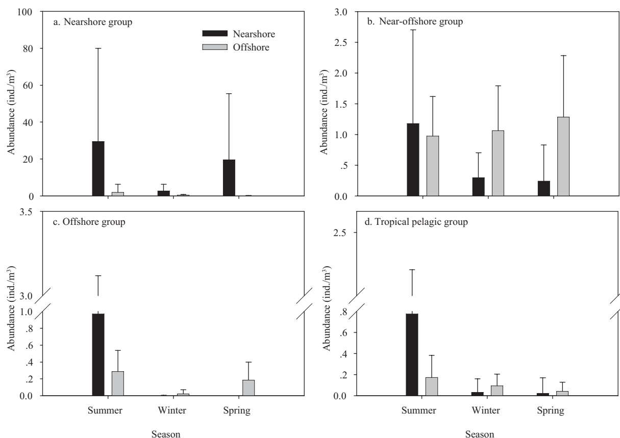
Fig.8 Seasonal variability in the abundance of nearshore, near-offshore, offshore and tropical pelagic groups in nearshore and offshore regions
