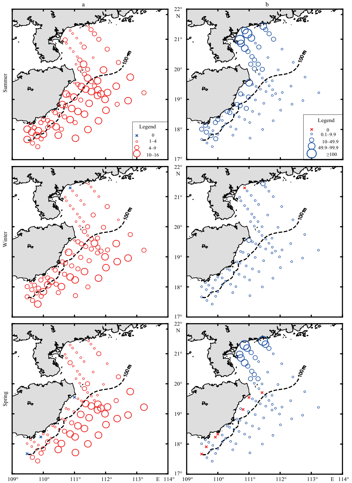
Fig.7 Species richness and abundance (ind./m 3 ) of siphonophores in the northern South China Sea during summer, winter and spring
