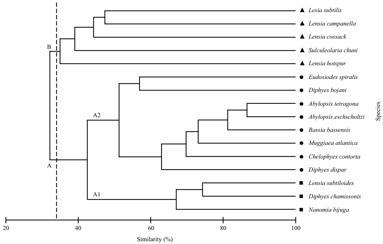
Fig.6 Dendrogram, based on the Bray-Curtis Similarity Index, of the siphonophores species with occurrence >25%
