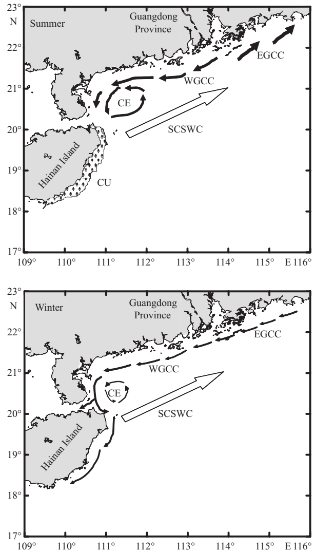
Fig.1 Sketch map of ocean currents in the study area during summer and winter
