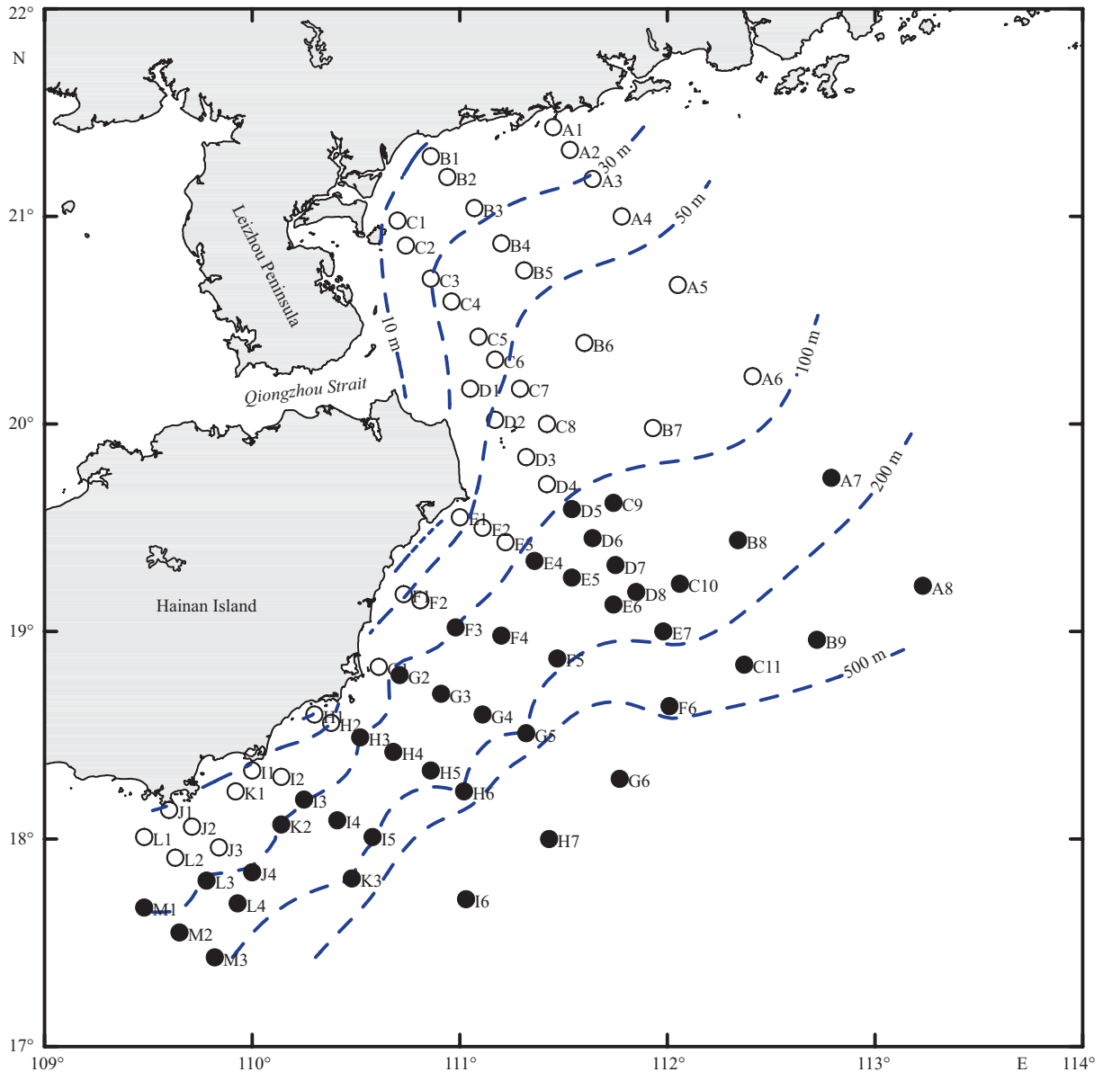
Fig.2 Map showing the positions of sampling stations (○: nearshore stations; ●: offshore stations) and underlying bathymetry on the northwest continental shelf of the South China Sea
