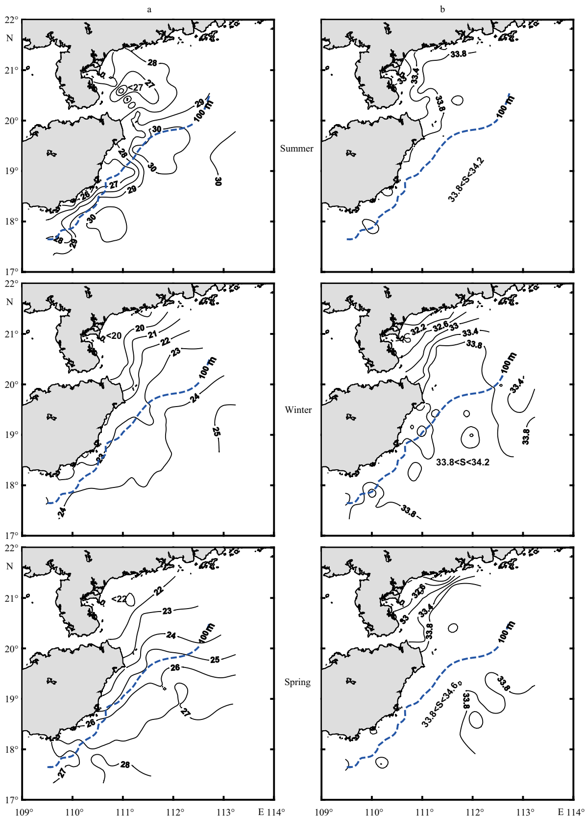
Fig.3 Horizontal distribution of surface sea temperature (SST, °C) and salinity (SSS) in the northern South China Sea during summer, winter and spring
