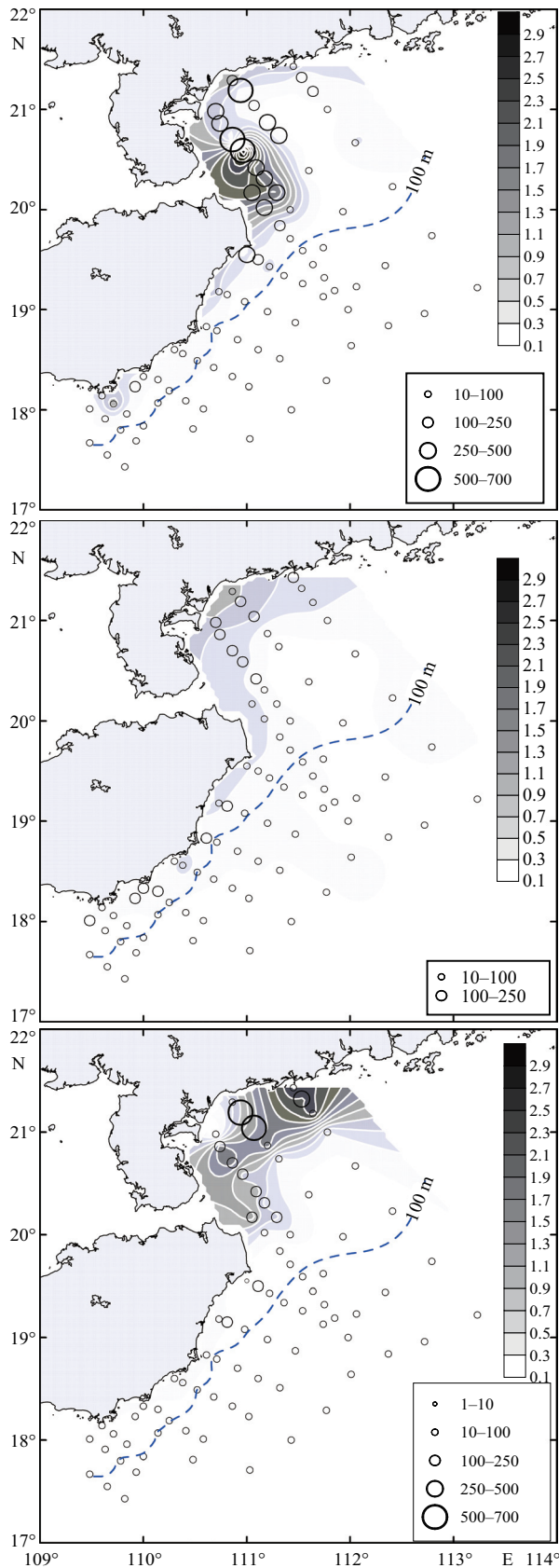
Fig.5 Chlorophyll a concentration ( \text{mg}/\text{m}^3 ) (gray scales) and abundance of copepods ( \text{ind.}/\text{m}^3 ) (blank circles) in summer, winter and spring
