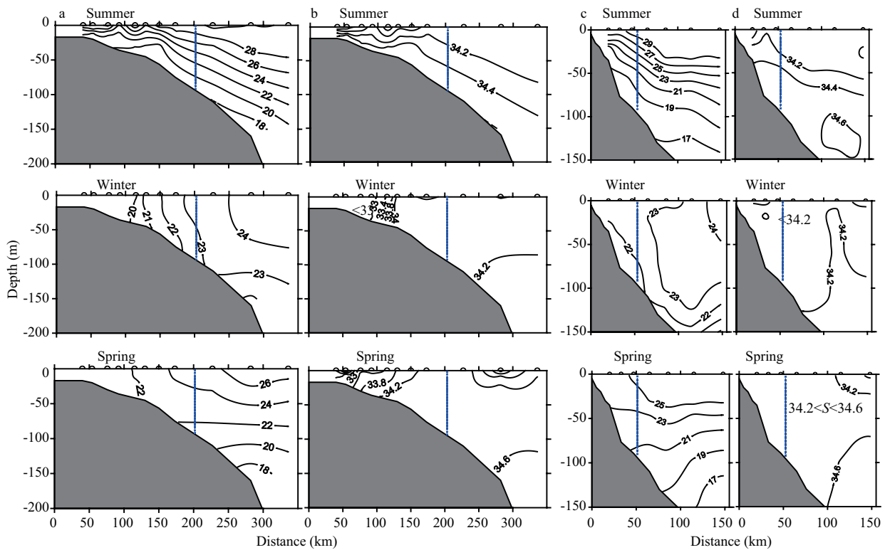
Fig.4 Vertical distribution of temperature (°C) and salinity at transects C and E during summer, winter and spring a and b: transect C temperature and salinity; c and d: transect E temperature and salinity. The dashed line indicates the 100 m depth contour.
