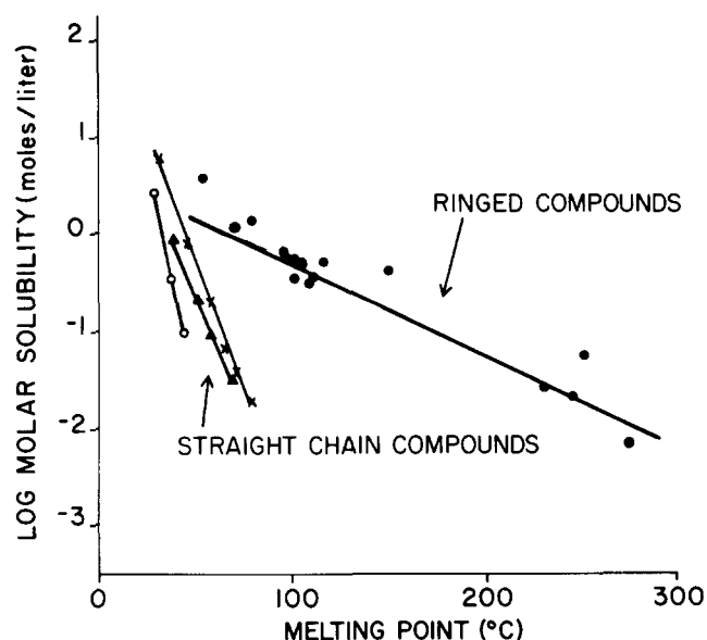
Fig. 2. The effect of melting point ( ^{\circ}\text{C} ) on the trioleoylglycerol solubility of crystalline nonelectrolyte compounds at 23^{\circ}\text{C} . (O) alkanes, ( \blacktriangle ) fatty alcohols, ( \times ) fatty acids, ( \bullet ) aromatic, chlorinated aromatic, and chlorinated aliphatic compounds. (See Tables 1 and 2).
