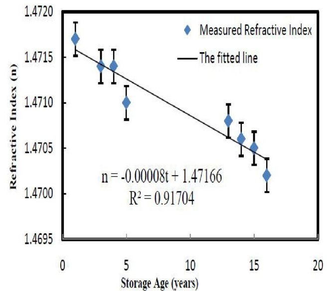
Figure 2 : Measured refractive index versus storage age of olive oil samples of L_1
