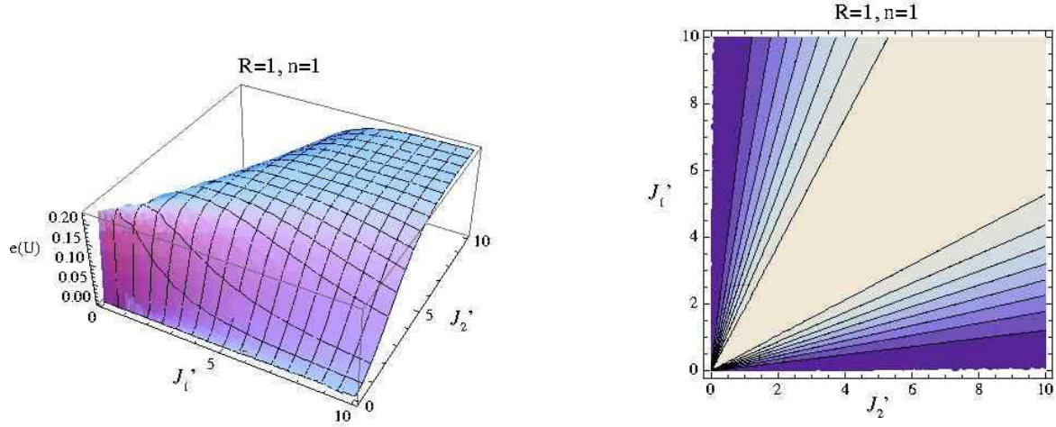
Figure 2. Average entangling power e(U) of the dynamic two qubit gate after the first revival n = 1 .
