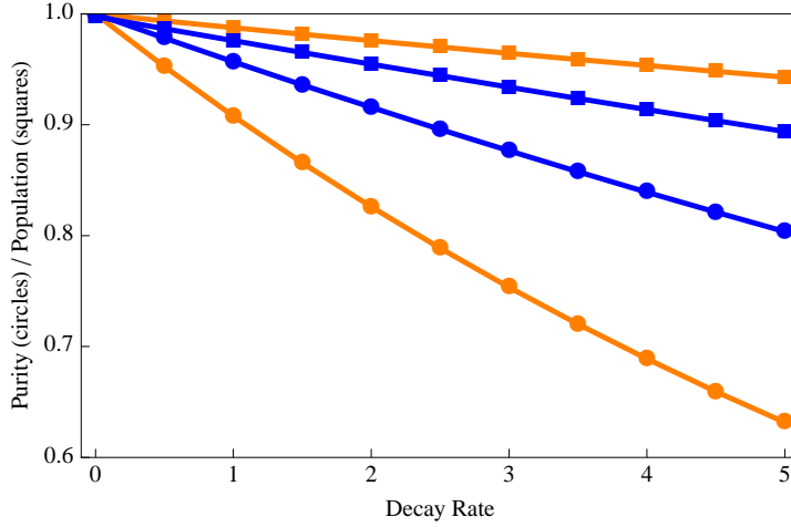
Figure 8. Comparison of final population in the computational basis (squares) and final purity of the system's density matrix (circles) for the adiabatic gate (orange) and the dynamic gate (blue). The decay rate is given in units of \text{ns}^{-1} and the system parameters are J_1 = J_2 = 0.05 \text{ ps}^{-1} and R = 1.2 . Typical laser control parameters have been used, such that both gates achieve an entangling power very close to the maximal value of e(U) \approx 0.22 .
