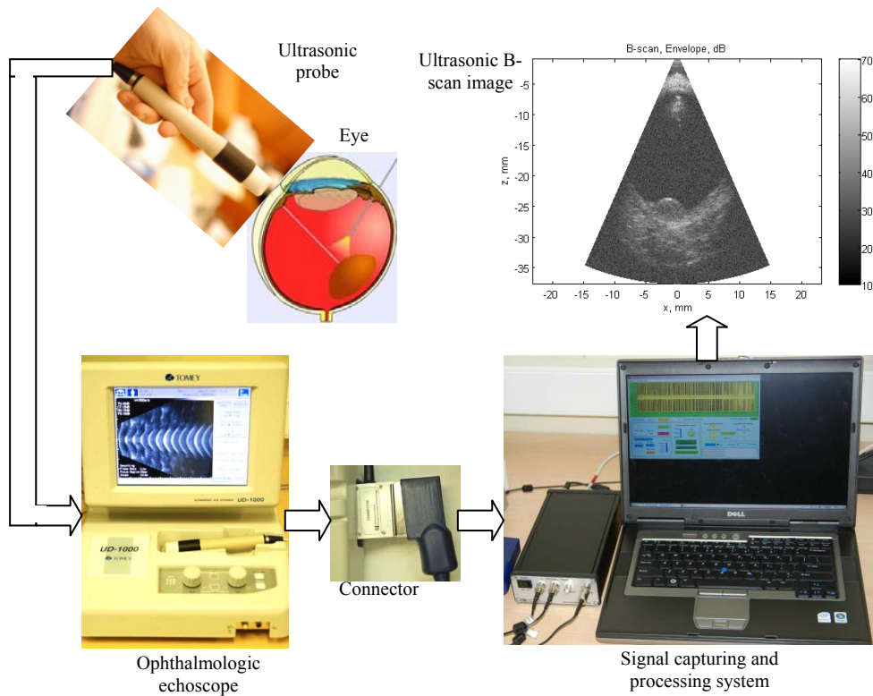
Fig.14. The experimental set-up for investigation of the eye tumours with conventional ophthalmological scanner and the ultrasonic imaging system-attachment.
