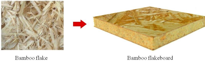
Figure 2. Bamboo flakeboard made from bamboo flake
