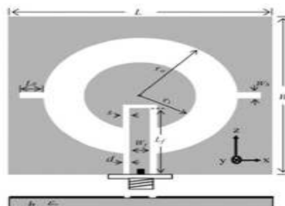
Figure 2: Geometry of the Proposed Broadband CPW-Fed Monopole Antenna with Parasitic Load
