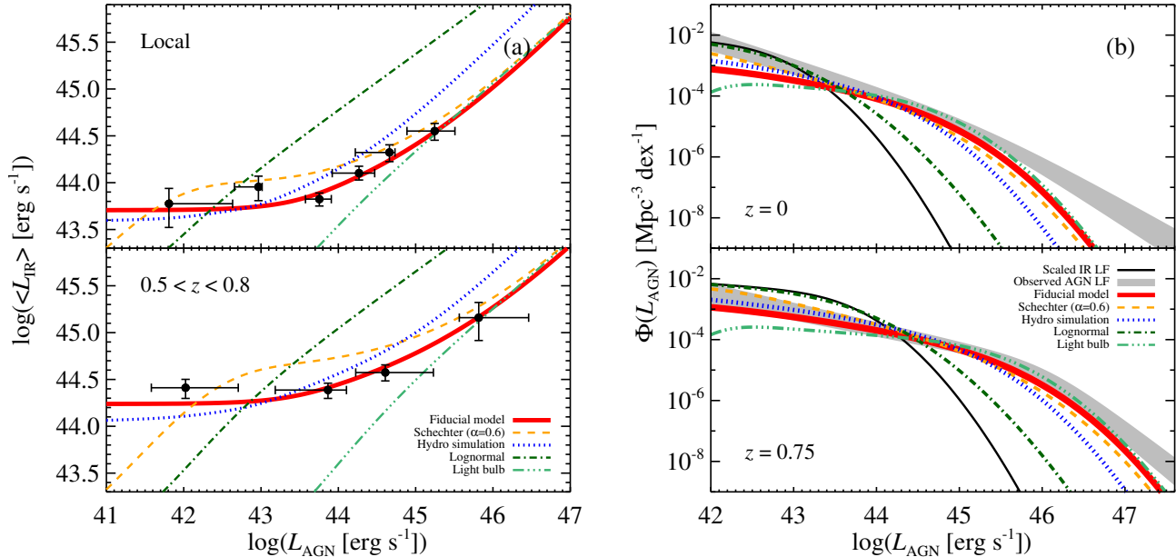
Figure 7. Comparison of the predictions of different AGN luminosity distributions for ( left ) the average SFR as a function of L_{\text{AGN}} , as in Figure 3(b), and ( right ) the AGN LF, as in Figure 5, for two representative redshift ranges. Both the distribution obtained by the Novak et al. (2011) simulation (blue dotted line) and our fiducial model (red solid line) can broadly reproduce both the observed trends with SF and the AGN LF. The steep observed AGN luminosity distribution at fixed stellar or BH mass (Hopkins & Hernquist 2009; Aird et al. 2012, modeled by the Schechter function with \alpha = 0.6 ) also produces a weak trend in the \langle \text{SFR} \rangle versus L_{\text{AGN}} (although less closely matching the data) and fits the AGN LF particularly well. In our simple picture, a “lognormal” luminosity distribution (Kauffmann & Heckman 2009) yields too strong a correlation between \langle \text{SFR} \rangle and L_{\text{AGN}} and fails to produce the high-luminosity tail of the AGN LF.
