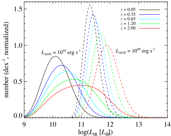
Figure 4. Distributions of L_{\text{IR}} predicted by our simple model for AGNs with moderate L_{\text{AGN}} = 10^{44} \text{ erg s}^{-1} (solid lines) and high L_{\text{AGN}} = 10^{46} \text{ erg s}^{-1} (dashed lines), evaluated at the same redshifts (coded by color) as in Figure 3. The distributions are normalized so that the integral under each curve is equal to 1. This figure demonstrates two key aspects of our model for the connection between SF and AGN activity: a shift to higher L_{\text{IR}} with increasing redshift at fixed L_{\text{AGN}} , and the narrow distribution of L_{\text{IR}} for high-luminosity AGNs compared to systems with lower L_{\text{AGN}} .
